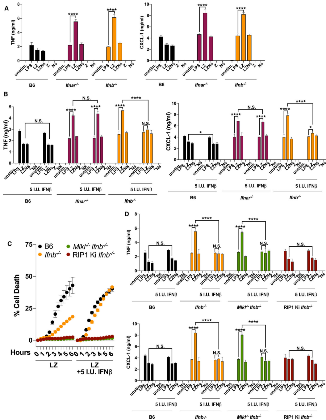
Figure 2. Constitutive IFN Signaling Downregulates RIPK-Dependent Inflammation
