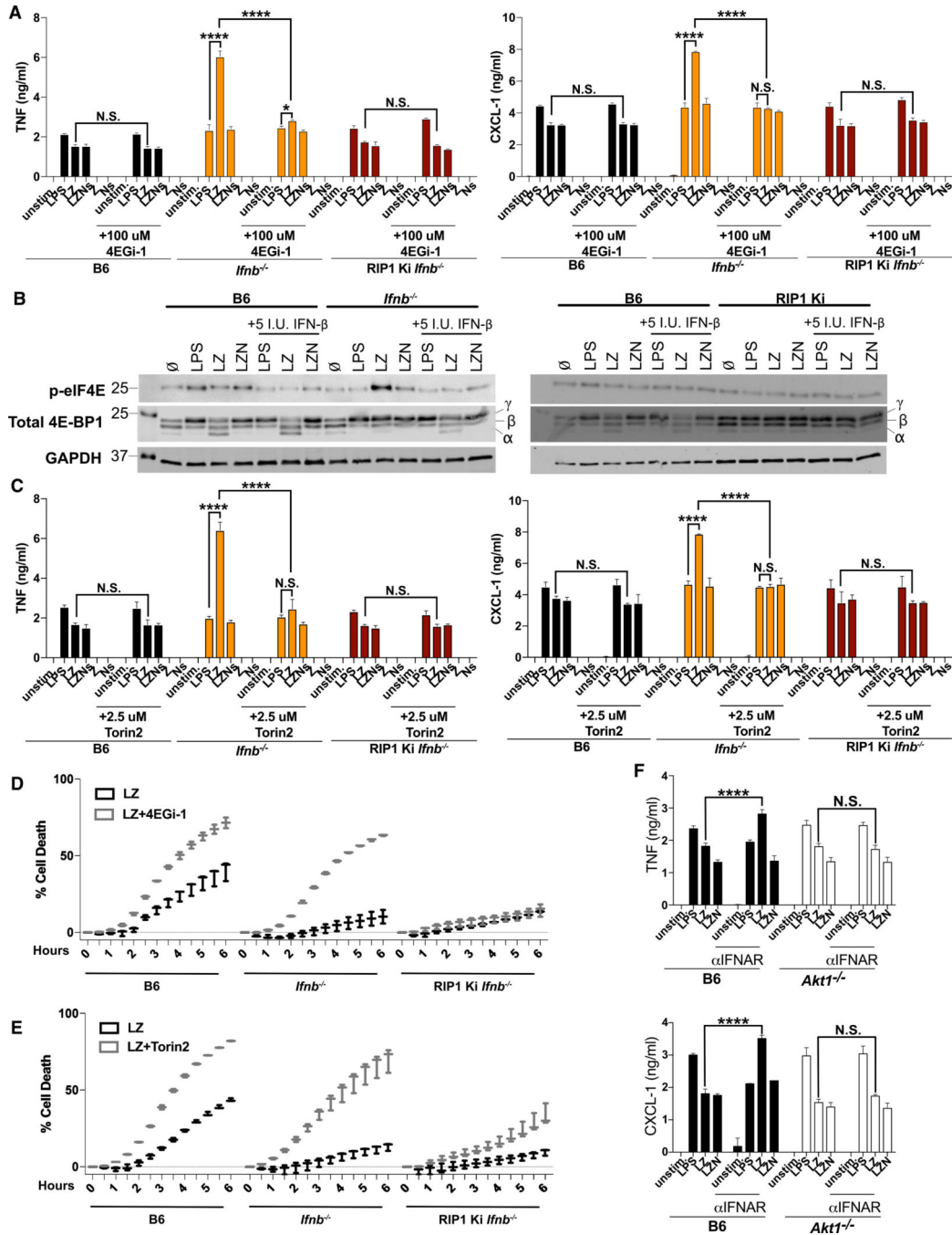
Figure 4. IFN Signaling Antagonizes RIPK in the Activation of eIF4E- and mTORC1-Mediated Translation
