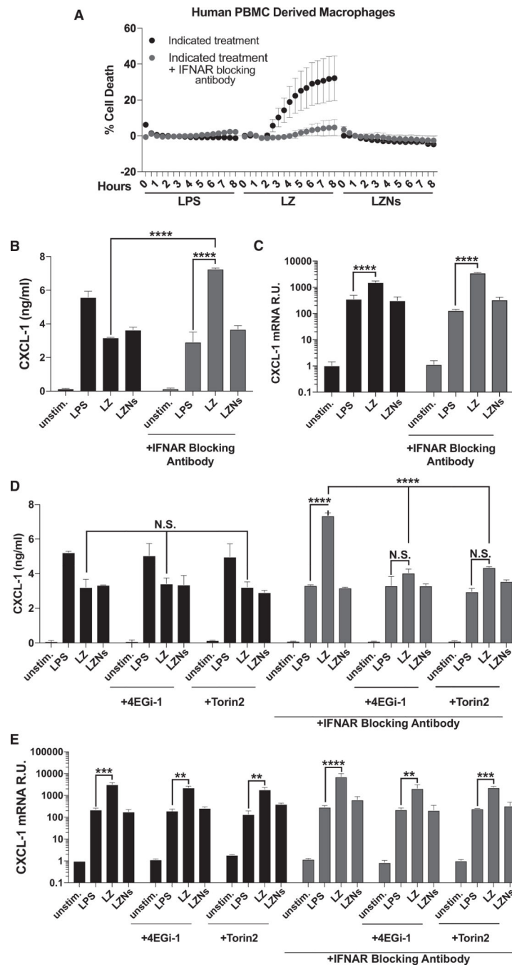
Figure 6. IFN Signaling Regulates RIPK-Dependent Cytokine Translation in Human PBMCs (A) Cell death as measured by propidium iodide incorporation over 8 h in human PBMC-derived macrophages stimulated as indicated ± overnight treatment with IFNAR-blocking antibody.
