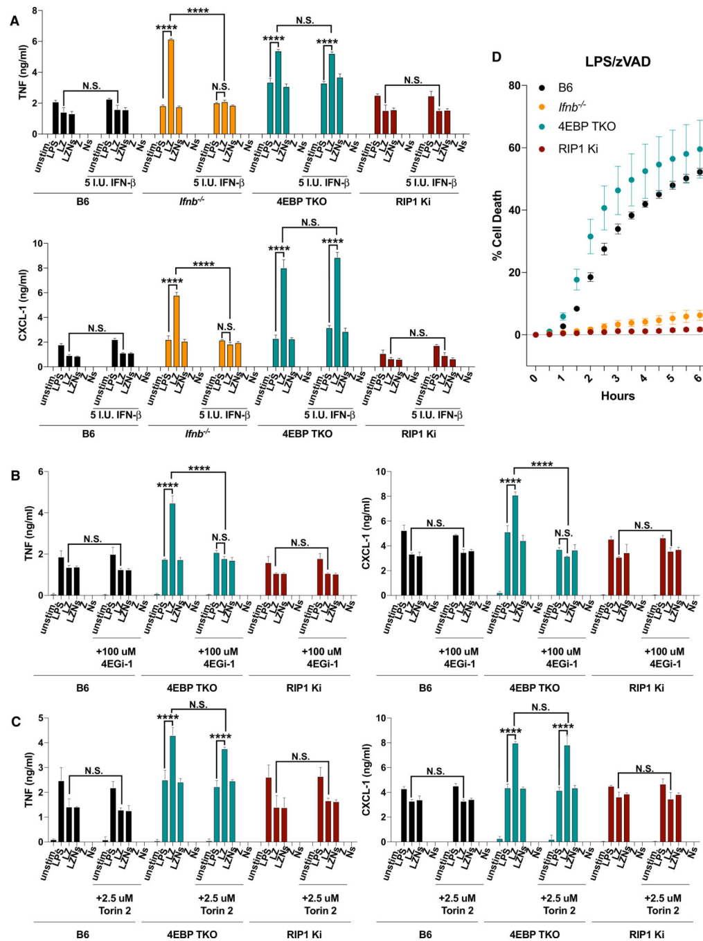
Figure 5. 4E-BP Activity Blocks RIPK-Dependent Cytokine Translation
