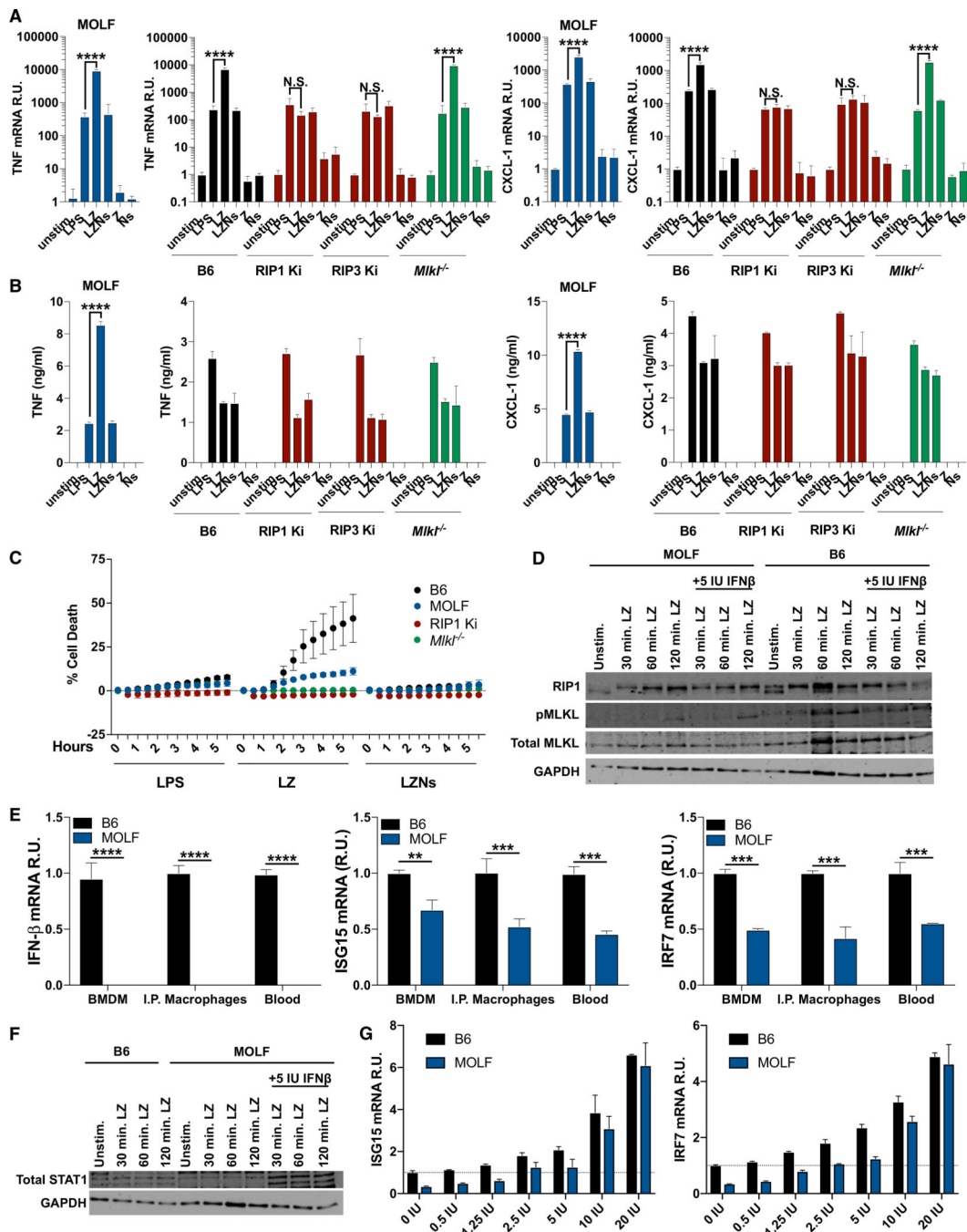
Figure 1. RIPK Promotes Cytokine mRNA and Protein Production in LPS-Activated MOLF Macrophages
