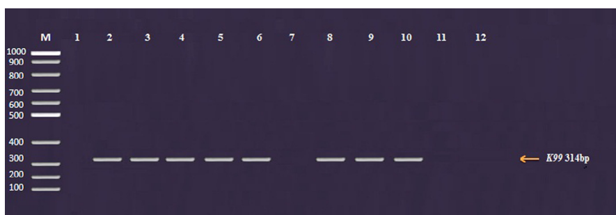
Fig. 2 – The PCR amplification of K99 virulence gene of E. coli showing positive amplicons at 314 bp. M: DNA size marker (100–1000 bp). Lane 1: Negative control. Lane 2: Positive control ( E. coli serogroup O 86 ). Lane (3–12): The tested serogroups (O 26 , O 44 , O 78 , O 86 , O 103 , O 111 , O 119 , O 127 , O 157 and O 158 , respectively).
