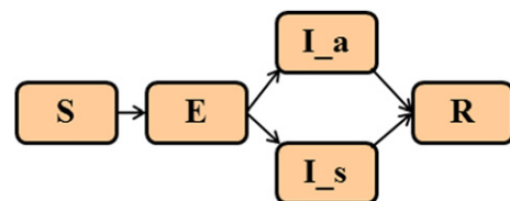
Figure 1 Mutually exclusive, allowable disease states of the model: susceptible (S), exposed (E), asymptotically infectious (I a ), symptomatically infectious (I s ), and recovered (R).
