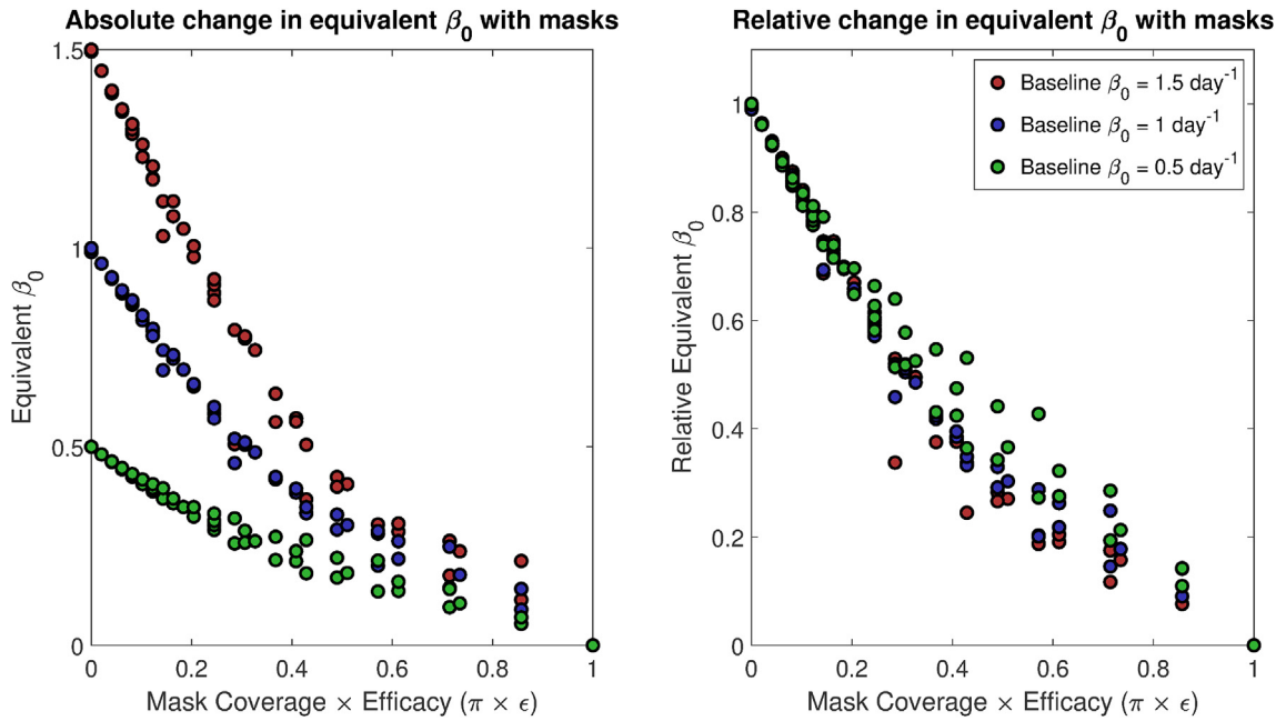
Fig. 2. Equivalent \beta_0, \tilde{\beta}_0 (infectious contact rate) under baseline model dynamics as a function of mask coverage \times efficacy, with the left panel giving the absolute value, and the right giving the ratio of \tilde{\beta}_0 to the true \beta_0 in the simulation with masks. That is, simulated epidemics are run with mask coverage and effectiveness ranging from 0 to 1, and the outcomes are tracked as synthetic data. The baseline model without mask dynamics is then fit to this synthetic data, with \beta_0 the trainable parameter; the resulting \beta_0 is the \tilde{\beta}_0 . This is done for simulated epidemics with a true \beta_0 of 1.5, 1, or 0.5 \text{day}^{-1} .
