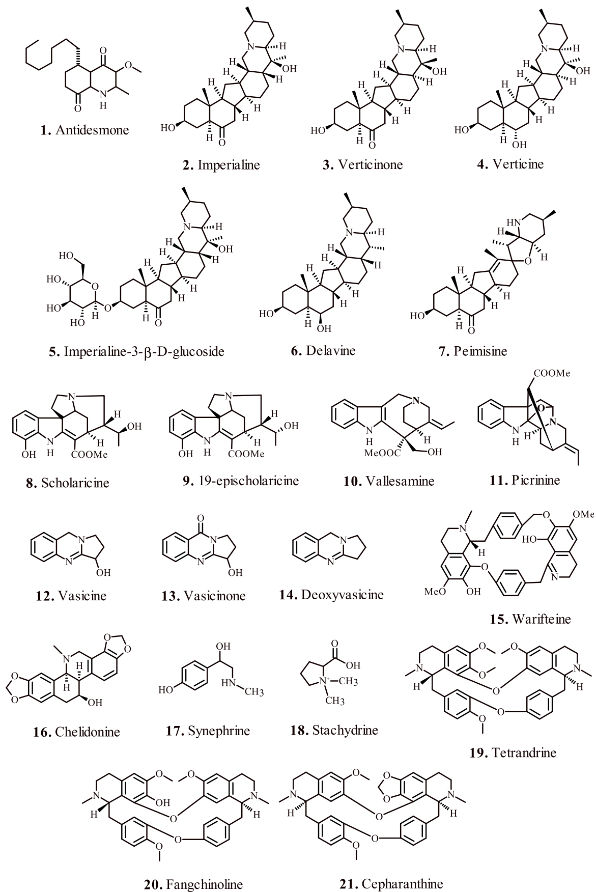
Fig. 2. Alkaloid based medicinal compounds for the treatment of respiratory disorders.
