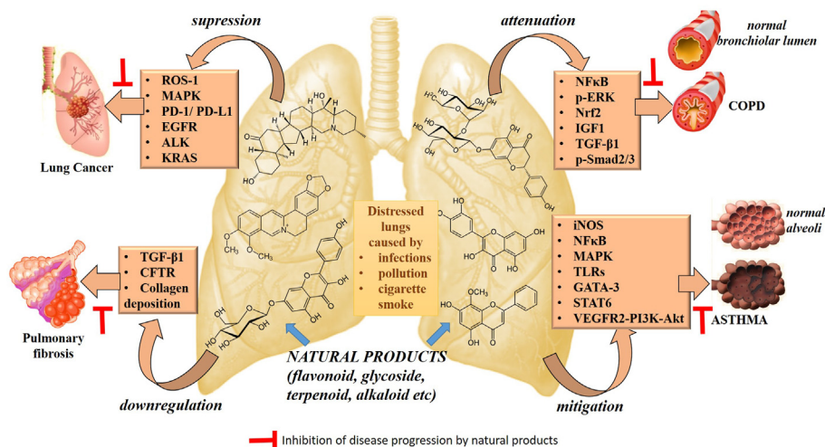
Fig. 1. Natural products targeting different cell signaling pathway.
