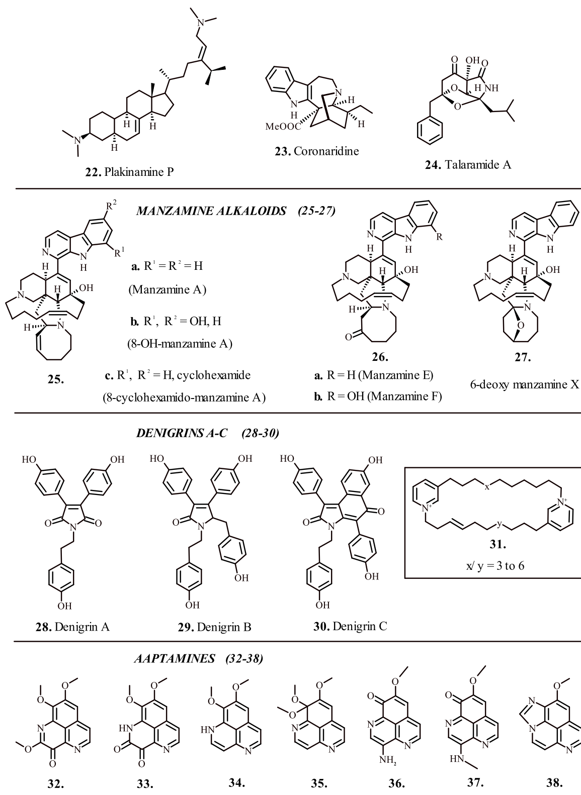
Fig. 3. Alkaloid based medicinal compounds for the treatment of tuberculosis.
