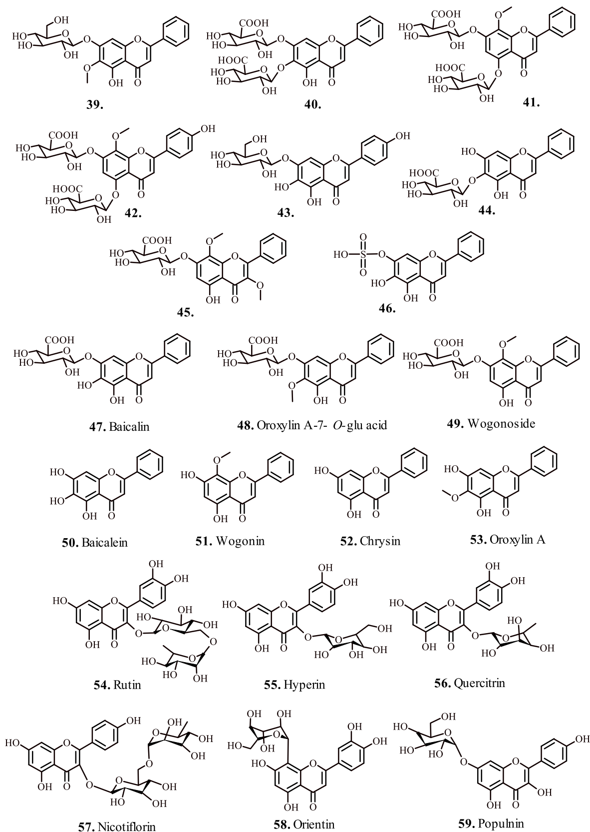
Fig. 5. Flavonoids for the treatment of respiratory disorders (b).
