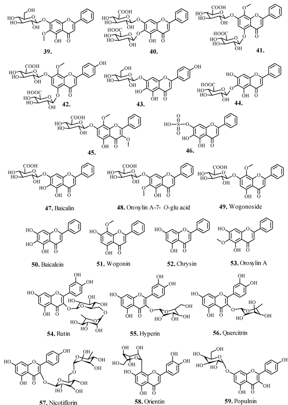
Fig. 4. Flavonoids for the treatment of respiratory disorders (a).
