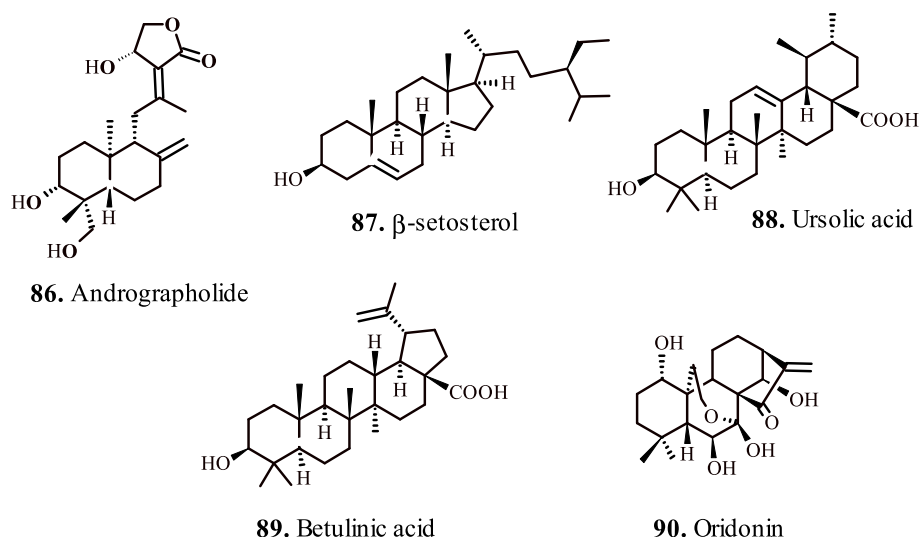
Fig. 7. Important terpenes for the treatment of respiratory disorders (b).
