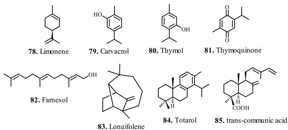
Fig. 6. Important terpenes for the treatment of respiratory disorders (a).
