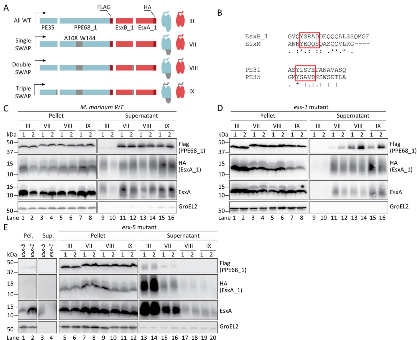
Figure 3. EsxA 1 is co-routed to ESX-5 by introducing the EspG 5 -binding domain of ESX-5 substrate PPE18 into PPE68 1 . A, schematic representation of the different constructs used in the secretion analysis. The introduced sequences of the ESX-5 substrates PE31/PPE18 are in gray. The FLAG tag (on PPE68 1 ) and HA tag (on EsxA 1 ) are shown in red. B, alignment of the swapped sequences containing the C-terminal secretion motifs of the ESX-5 substrates PE31 and EsxM and the ESX-1 substrates PE35 and EsxB 1 , respectively. The conserved secretion motif YXXX(D/E) are highlighted with red boxes. C–E, immunoblot analysis of EsxA 1 as detected with an HA antibody, PPE68 1 as probed with a FLAG antibody and endogenous and exogenous EsxA paralogs using an EsxA antibody and intracellular GroEL2 by an GroEL2 antibody, in pellet and supernatant fractions. Different derivatives of PE35/PPE68 1 /EsxB 1 /EsxA 1 were tested in WT M. marinum (C), an eccB mutant ( esx-1 mutant; D), and an eccC knockout strain ( esx-5 mutant; E). Equivalent OD units of cell pellets (0.2 OD unit) and culture supernatants (0.5 OD unit) are shown. Numbers indicate two independent M. marinum colonies carrying the same construct.
