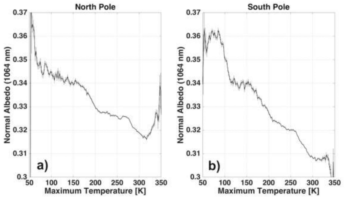
Figure 2. Average reflectance plotted as functions of maximum temperature for the (a) North and (b) South poles. Maximum temperature bin width=1K. Average reflectance curves are plotted with 2\sigma standard error of the mean.
