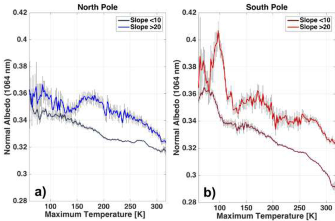
Figure 4. Average 1064 nm reflectance as a function of maximum temperature for low slope (slope < 10^\circ ) and high slope (slope > 20^\circ ) areas for the North ( a ) and South ( b ) polar regions. Maximum Temperature bin width=2K. Reflectance average plotted with 2\sigma errors (standard error of the mean). [1.5 column]
