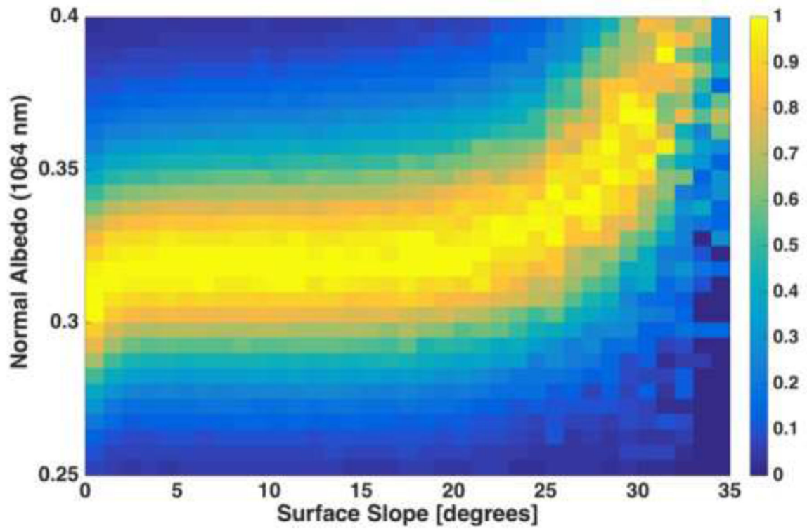
Figure 3. Two-dimensional histogram that displays mode-normalized LOLA reflectance distribution as a function of surface slope for the North and South pole. Reflectance bin width=0.005 and slope bin width=1 degree . The strong influence of surface slope is a potential source of temperature-independent bias on the reflectance-temperature relationships observed in the polar regions. [1 column]
