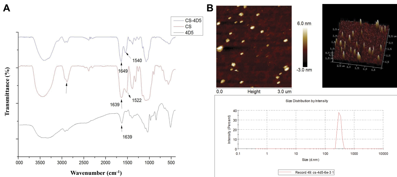
Figure 1 Structural characterization of CS-4D5 and CS-4D5/6e. (A) Infrared spectra of CS, 4D5, and CS-4D5. (B) AFM images and Marv particle size distribution chart of CS-4D5/6e.
