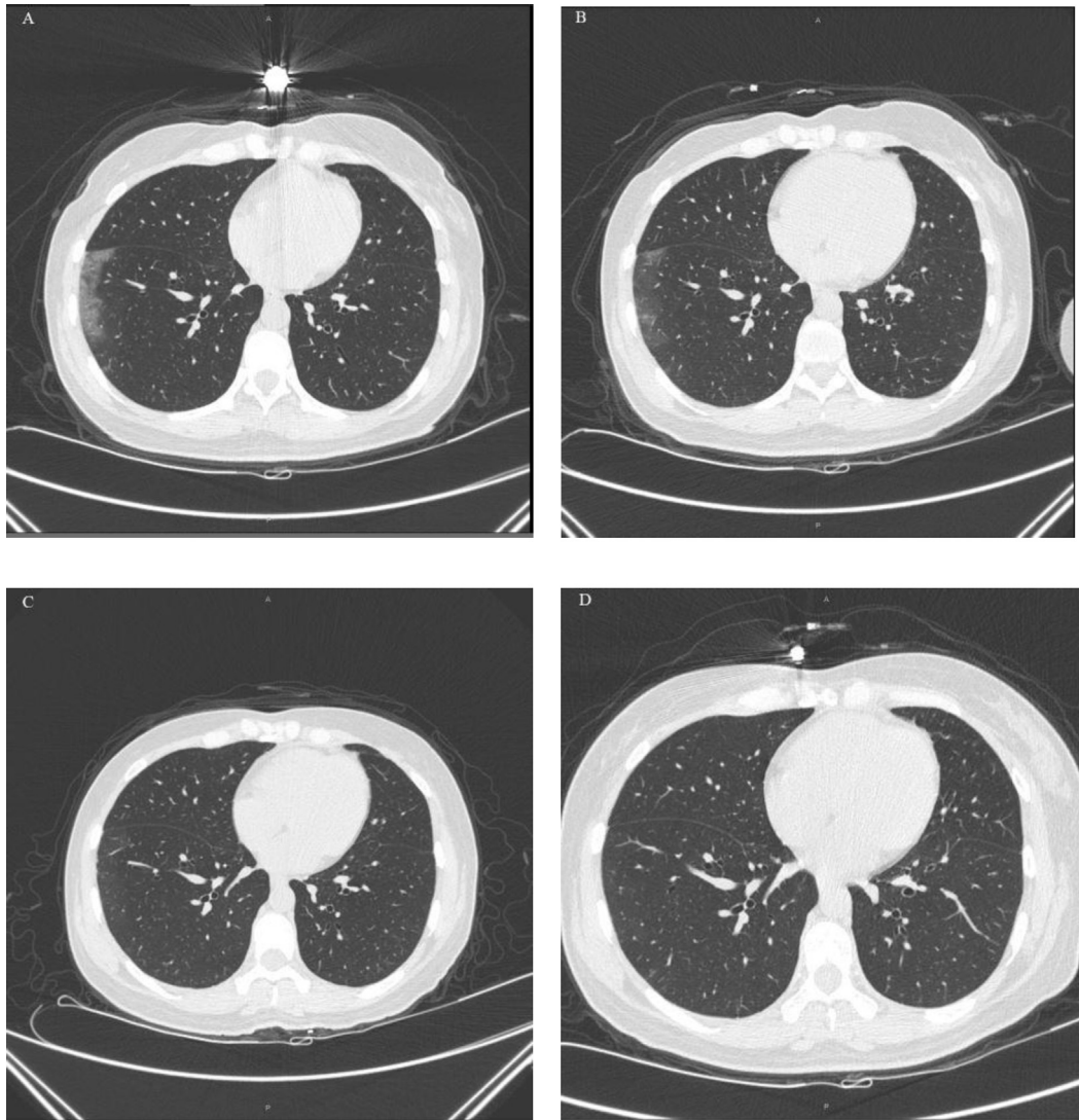
Fig. 2. Dynamic changes of the chest CT of an asymptomatic patient obtained on February 5(A), February 8(B), February 14(C) and February 19(D).
