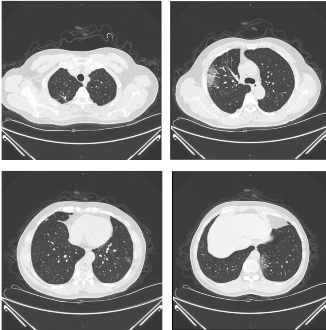
Fig. 1. Representative lung images of an asymptomatic patient in which lesions developed in multiple lobes, most of which were subpleural ground-glass opacity co-existed with consolidation.
