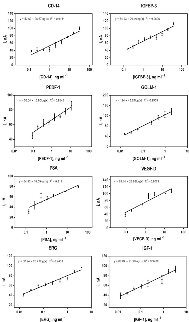
Fig. 2. Immunoarray calibration plots using amperometric responses for PSA, VEGF, ERG, IGF-I, IGFBP-3, CD-14, PEDF and GOLM-1 at -0.2 V vs Ag/AgCl developed by injecting 1 mM HQ and 0.1 mM \text{H}_2\text{O}_2 after capturing analyte \text{Ab}_2\text{-HRP-MB-Ag} bioconjugates on modified carbon electrode surfaces contained within the microfluidic device detection chambers. Protein standards were diluted 5X in calf serum, to mimic a complex sample matrix. Error bars represent the range ( n=2 ) for the two electrodes in each immunoarray designed to detect the protein.
