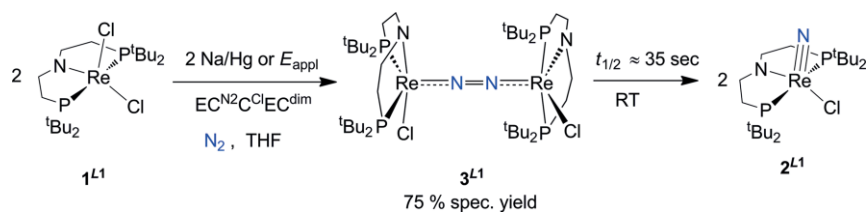
Scheme 2. (Electro)chemical N 2 -activation from [ReCl 2 (L1)] ( 1 L1 ) into [Re(N)Cl(L1)] ( 2 L1 ) via the N 2 -bound dimeric intermediate EC^{N_2}C^ClEC^{dim} type mechanism.
