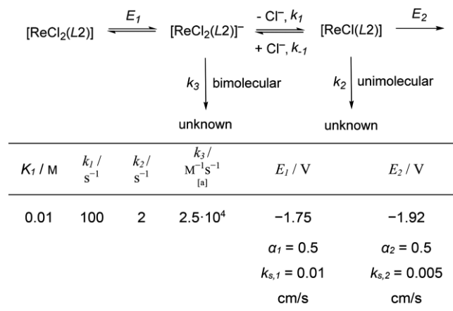
Scheme 5. Minimum kinetic model for the digital simulation of the electrochemical reduction of 1 L2 under Ar and thermodynamic and kinetic parameters (formal potentials, rate constants, and electron transfer parameters) obtained from CV data simulation; [a] for bimolecular decay of [ReCl 2 (L2)] - .
