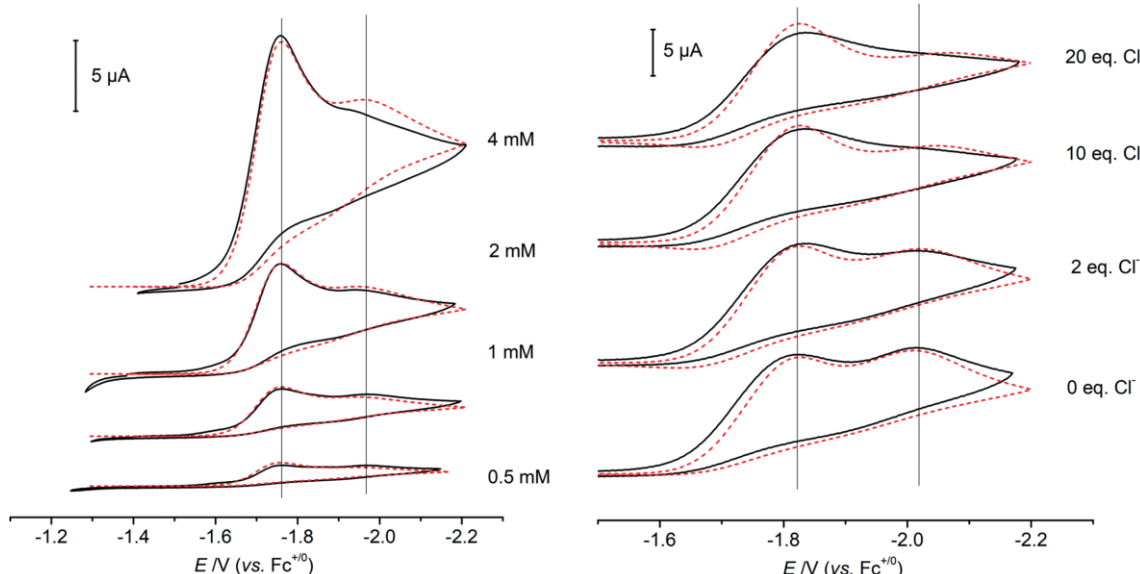
Figure 3. Experimental (black lines) and simulated (red dashed lines) CV data [0.2 M ( n Bu 4 N)PF 6 in THF] of 1 L2 under Ar; mechanism and simulation parameters according to Scheme 5. Left: Concentration dependent data, \nu = 0.1 V s -1 . Right: Chloride dependent data, \nu = 0.5 V s -1 .
