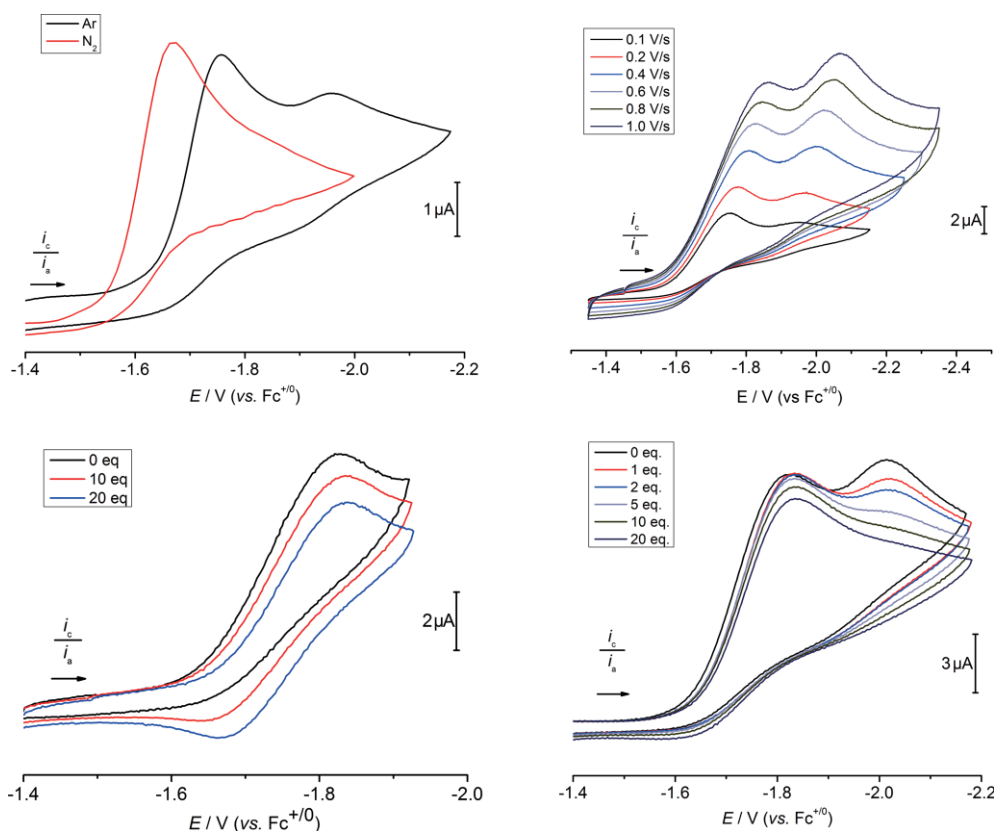
Figure 2. CVs of \mathbf{1}^{\text{L}2} . Top Left: Ar (black) and \text{N}_2 (red) at \nu = 0.1 V \text{s}^{-1} . Top Right: Scan rate dependence under Ar. Bottom Left: Under Ar, in the presence of varying amounts of (n\text{Bu}_4\text{N})\text{Cl} ( \nu = 0.5 V \text{s}^{-1} ). Bottom Right: Under Ar, in the presence of varying amounts of (n\text{Bu}_4\text{N})\text{PF}_6 ( \nu = 0.5 V \text{s}^{-1} ). General conditions: 1.0 mM \mathbf{1}^{\text{L}2} in THF, 0.2 M (n\text{Bu}_4\text{N})\text{PF}_6 .
