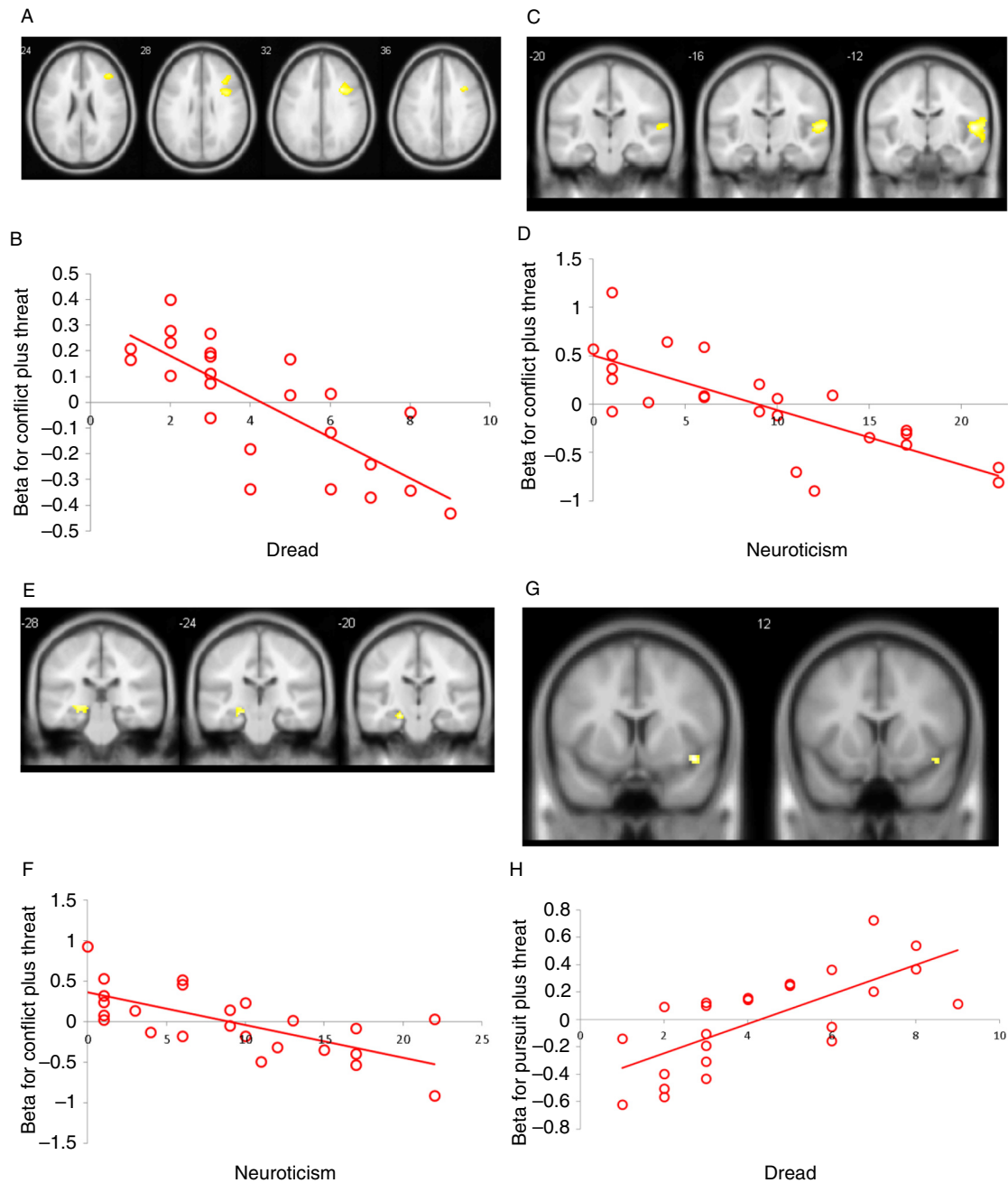
Figure 4. Scatterplots showing effect on BOLD signal of inter-individual differences in dread elicited by threat of electric shock and also neuroticism (as measured by the Eysenck Personality Questionnaire). (A, B) Right dorsolateral prefrontal cortex [32, 12, 34]. (C, D) Right superior temporal gyrus [52, -12, 8]. (E, F) Left hippocampus [-22, -22, -15]. (G, H) Operculum/right posterior insula [48, 8, -12]. Each point represents an individual's response on the self-report measures.
