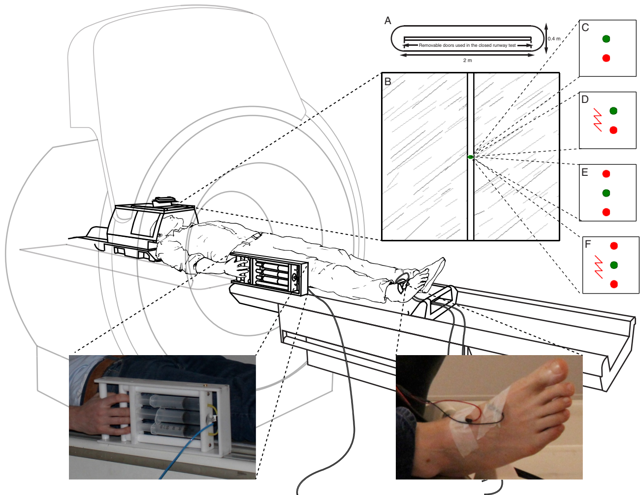
Figure 1. (A) The Mouse Defense Test Battery. (B) The Joystick Operated Runway Task. A force-sensing interface controls the speed of a green dot cursor pursued along a runway by a red dot cursor capable of inflicting electric shock. The task comprised 12 trials each of pursuit (C), pursuit plus threat of electric shock (D), goal conflict (E), goal conflict plus threat of electric shock (F). Illustration by Nick Boon.
