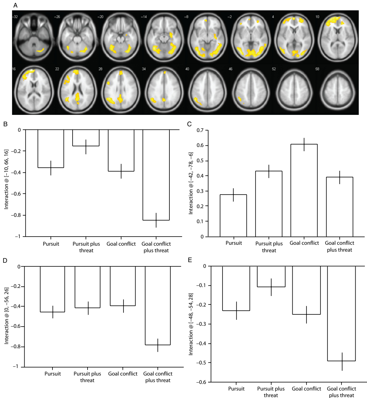
Figure 2. (A) Statistical parametric maps illustrating blood oxygen level-dependent (BOLD) responses for the Condition \times Threat interaction. (B) Parameter estimates for activity in the medial prefrontal gyrus [-10, 66, 16]; (C) inferior occipital gyrus [-42, -78, -6]; (D) angular gyrus [0, -56, 26]; (E) precuneus [-48, -54, 28]. All regions survive whole-brain family-wise error correction on the basis of cluster extent ( p_{\text{FWE}} < 0.05 ) with a default cluster-forming threshold of p < 0.001 . Error bars represent 1 SEM.
