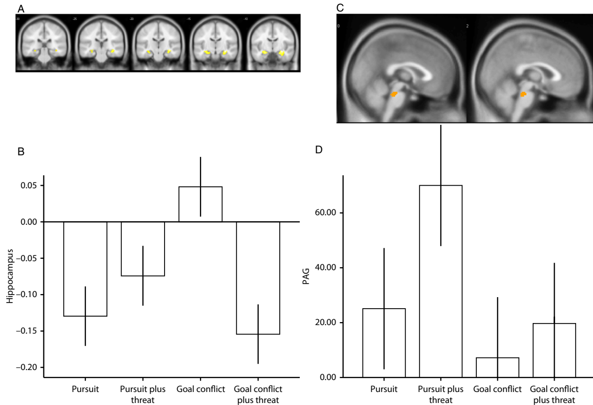
Figure 3. (A) Statistical parametric map illustrating blood oxygen level-dependent (BOLD) responses in the anterior hippocampi during the goal conflict condition (shown at an uncorrected voxel threshold of p < 0.005 for display purposes). (B) Parameter estimates for activity in the right anterior hippocampus [32, -14, -12] during the four task conditions. (C) BOLD responses in the periaqueductal gray (PAG) at the point of peak threat proximity during pursuit plus threat of electric shock (shown at an uncorrected voxel threshold p < 0.01 for display purposes). (D) Mean BOLD activity in PAG for the task conditions [6 -28 -28]. Error bars represent 1 SEM; the y-axis displays beta values that reflect scaling factors for the peak threat value to fit the residual after fitting the mean.
