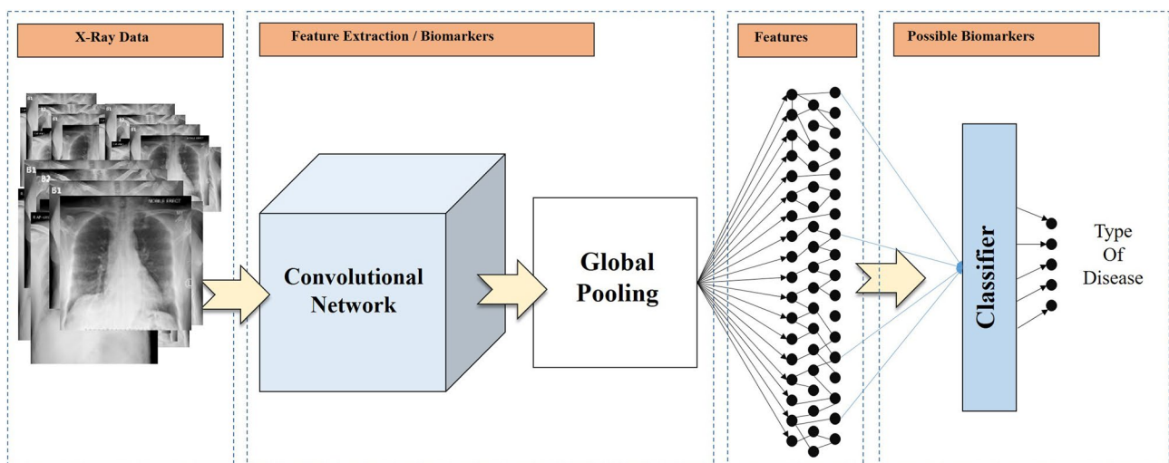
Fig. 1 Overview of the feature extraction process
