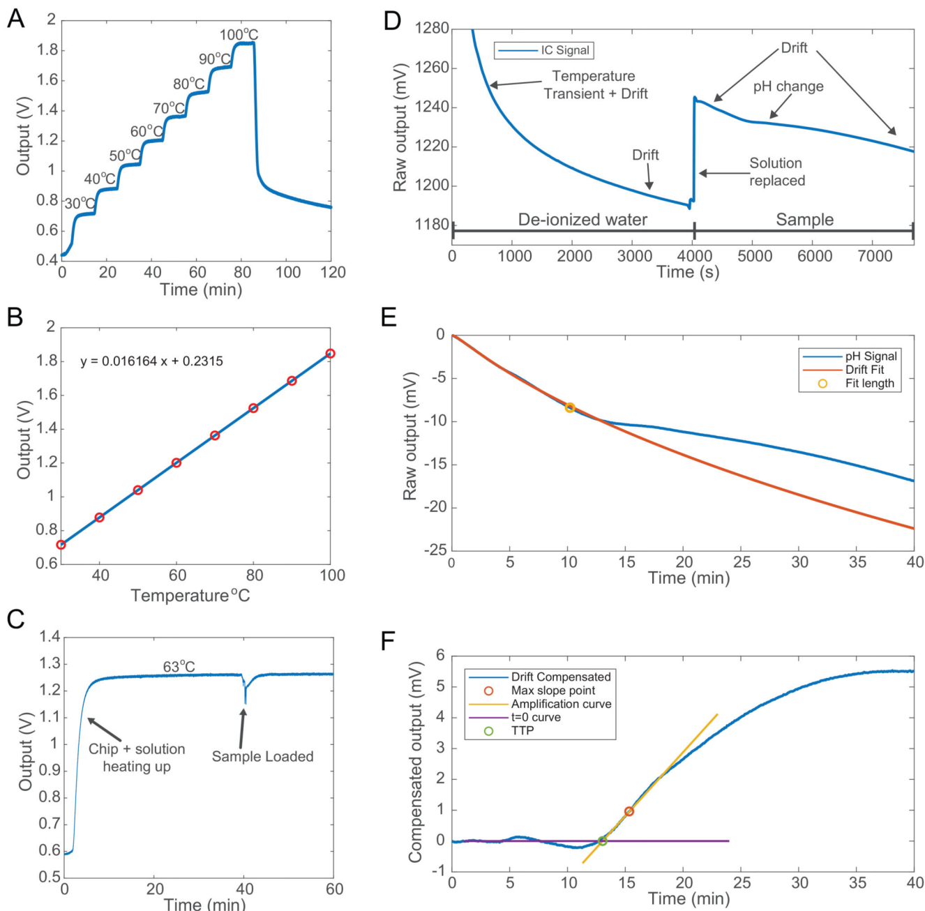
Figure 2. Temperature Sensor and Data Processing
