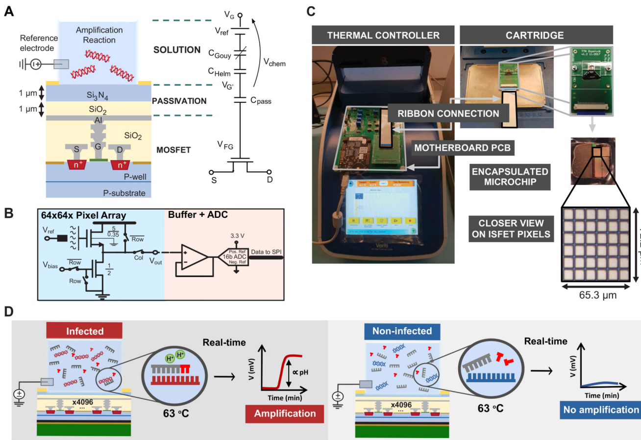
Figure 1. Experimental configuration using the Lab-on-Chip platform.
