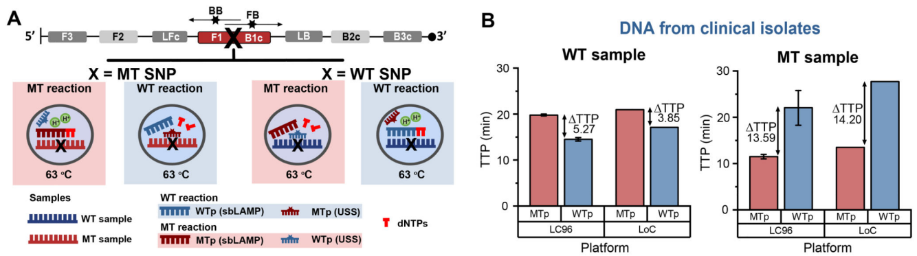
Figure 5. Lab-on-Chip detection of C580Y SNP associated to P. falciparum artemisinin-resistance.
