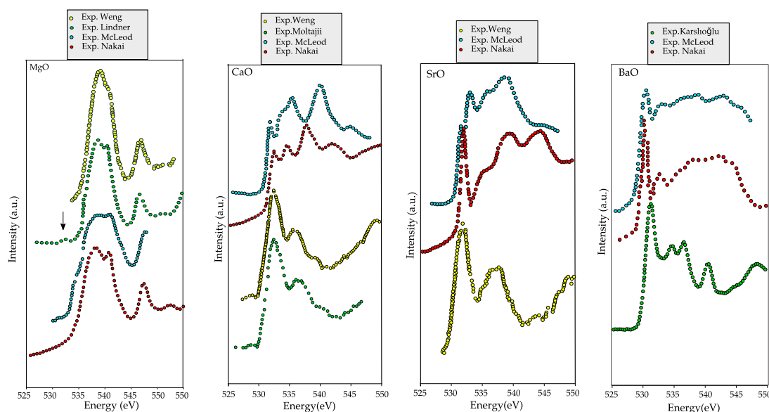
Figure 24. Oxygen K-edge spectra of alkaline earth oxides showing discrepancies between the experiments: MgO, 232,234,235,237 CaO, 232–235 SrO, 232,234,235 and BaO. 232,234,236
