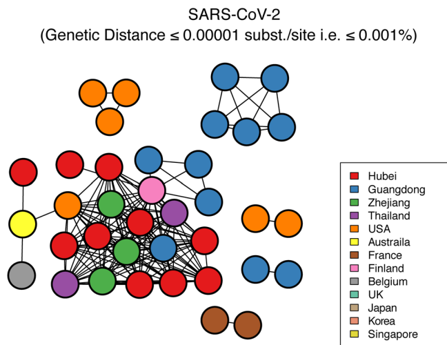
FIGURE 5 Transmission clusters of severe acute respiratory syndrome coronavirus 2 (SARS-CoV-2). Structure of inferred SARS-CoV-2 transmission clusters from “dataset_70” using genetic distances of <math><0.001\%</math> substitutions/site is shown. Nodes (circles) represent connected individuals in overall network, and putative transmission linkages are represented by edges (lines). Nodes are color-coded by sampling locations
