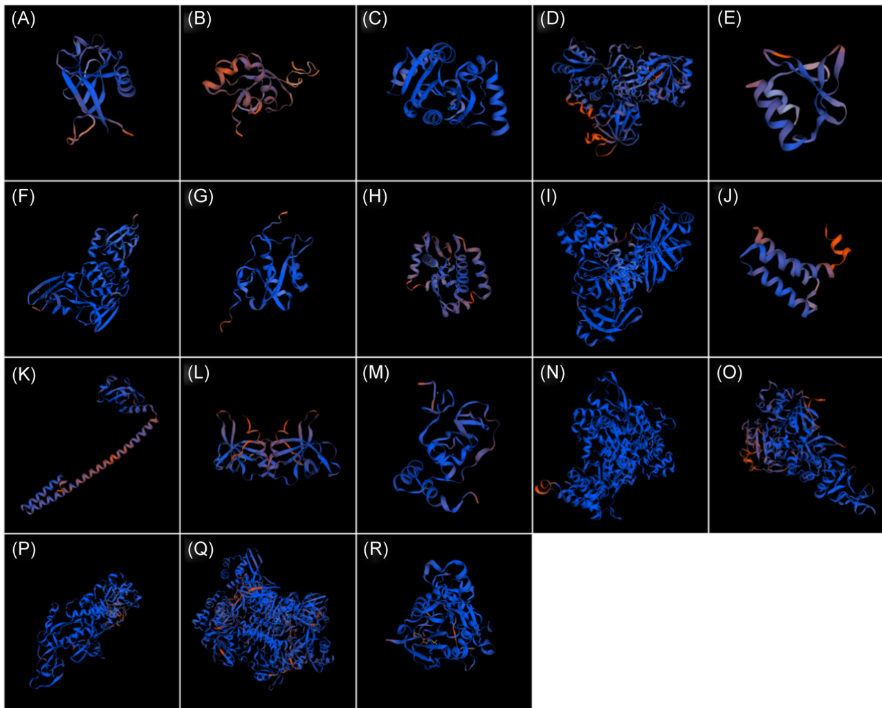
FIGURE 1 Cartoon displayed models of ORF1ab related proteins constructed based on (A) 2HSX_A, (B) 2IDY_A, (C) 2ACF_A, (D) 2WCT_A, (E) 2KAF_A, (F) 5T16_A, (G) 2K87_A, (H) 3VCB_A, (I) 5B6O_A, (J) 2AHM_A, (K) 2AHM_G, (L) 1UW7_A, (M) 5C8S_A, (N) 6NUR_A, (O) 6JYT_A, (P) 5C8S_B, (Q) 2H85_A, and (R) 3R24_A
