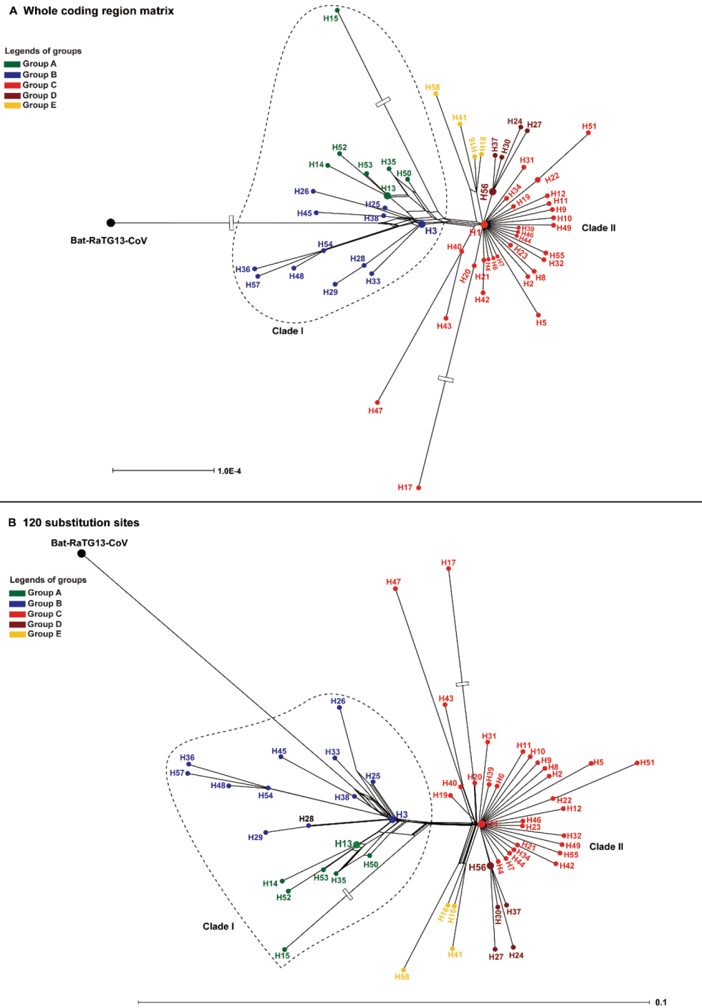
Figure 4 Phylogenetic networks of 58 haplotypes of SARS-CoV-2 with the outgroup bat-RaTG13-CoV using the whole coding region matrix (A) and 120 substitution sites (B), referring to all variable sites of coding regions in SARS-CoV-2 haplotypes The bottom scale bars represent the number of substitutions per site. The open box on branches of bat-RaTG13-CoV (A), H15 (A, B), and H17 (A, B) indicating a long branch was clipped.
