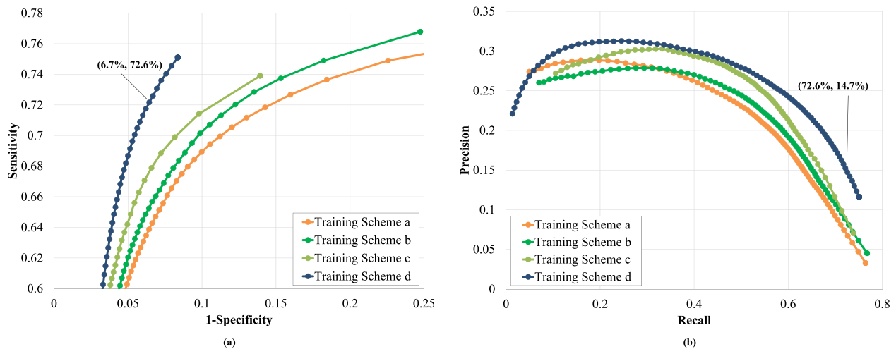
Fig. 2 The image-based performance of AI-doscopist on Dataset B under different training schemes. a the Receiver Operating Characteristic curves and b the Precision–Recall curves. In Training Scheme a, AI-doscopist learnt only the spatial features from a random subset of 33,819 original colonoscopy images. In Scheme b, the training set was enlarged to a random subset of 119,703 original colonoscopy and non-medical images. In Scheme c, AI-doscopist learnt both the spatial and temporal features from a random subset of 119,703 original colonoscopy and non-medical images. In Training Scheme d, the spatial and temporal features were learnt from a larger, random subset of 191,493 colonoscopy and non-medical images. A total of 34,469 images were used for validation in each case.
