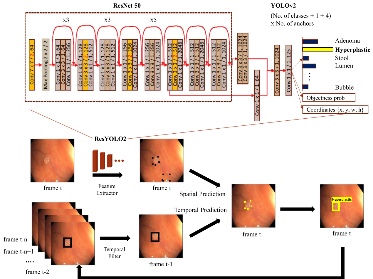
Fig. 4 An overview of the algorithm design of AI-doscopist. AI-doscopist was constructed based on ResNet50, YOLOv2, and a temporal tracker. The model was found to perform reasonably well with a good trade-off between speed and accuracy in earlier studies. The feature extractor was adopted from a modified version of ResNet50. A one-stage object detector, YOLOv2, was selected for localising objects in each image in real-time. Predicted boxes that were unlikely polyp were removed and overlapped predicted boxes were combined using the non-maximum suppression method. Temporal information was incorporated by using the majority votes of the prediction results within a sliding window.
