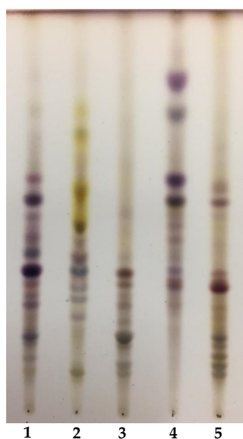
Figure 1. TLC of the five saponin extracts. 1: M. heyniiana ; 2: M. hybrida ; 3: M. lupulina ; 4: M. murex ; 5: M. truncatula . Spots were visualized by Liebermann–Burckard reagent.
