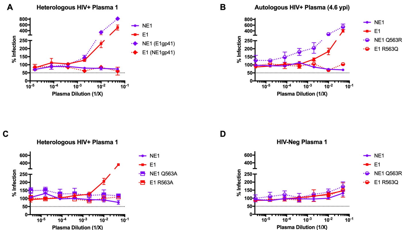
Fig 3. A single-residue change in the gp41 region (Q563R) of Env E1 is responsible for the increased infection observed specifically with HIV-positive plasma.
