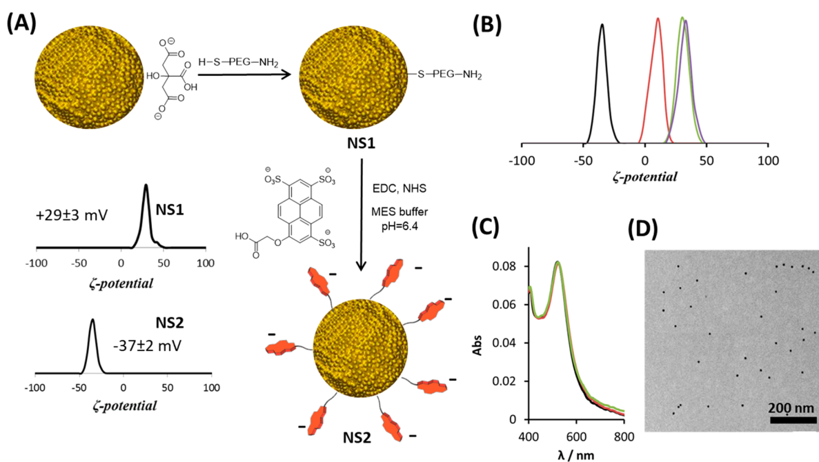
Figure 2. NS2 synthesis and evaluation of its interaction with cage A. (A) Synthesis scheme and Zp characterization of NS1 and NS2. (B) Zp distributions for NS2 after addition of cage A. (black) 2 \times 10^{11} particles/mL suspension of NS2 in Milli-Q water ( -37 \pm 2 mV). (red) After addition of 0.3 \mu\text{M} of A ( +8 \pm 2 mV). (green) After addition of 3 \mu\text{M} of A ( +31 \pm 2 mV). (purple) After addition of 5 \mu\text{M} of A ( +32 \pm 3 mV). (C) UV-Vis spectra of NS2 ( 1.5 \times 10^{11} particles/mL) before and after addition of cage A. (black) NS2 in Milli-Q water. (red) After addition of 5 \mu\text{M} of A. (green) After addition of 10 \mu\text{M} of A. (D) Representative TEM corresponding to the sample with the red spectrum in (C).
