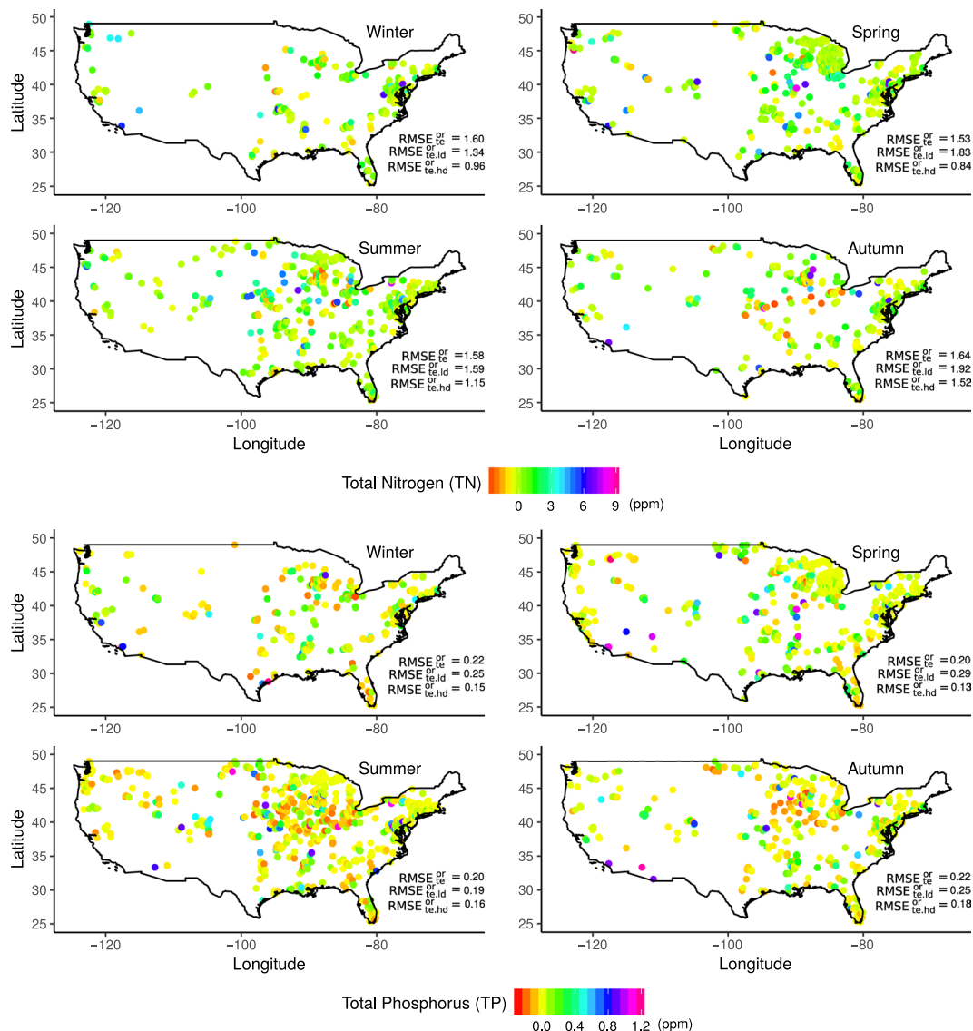
Fig. 4 Residual maps for TN and TP. Residuals are computed using the testing sub-dataset (observations minus predictions). In each maps is also reported the RMSE_{te}^{or} for the testing sub-daset in ppm, RMSE_{te.ld}^{or} and RMSE_{te.hd}^{or} using observation in the low/high density, respectively.
