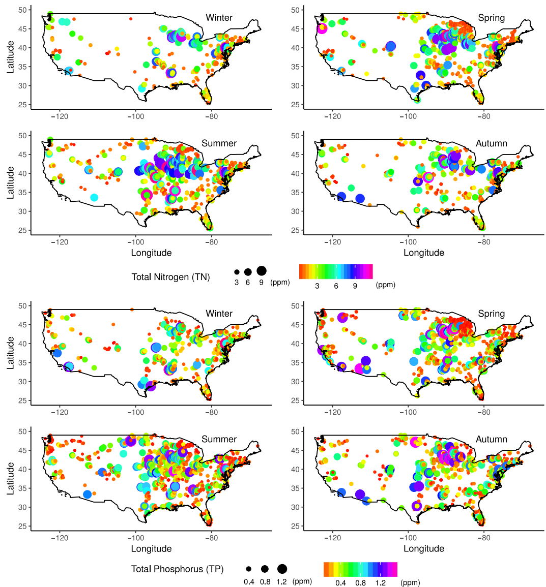
Fig. 1 Spatio-temporal distribution of TN and TP. Spatial and seasonal distribution of the Water Quality Portal's stations. The Total Nitrogen (TN) and Total Phosphorus (TP) seasonal mean for each station is labelled by a colour circle which also increase in size in accordance to the value TN and TP values.
