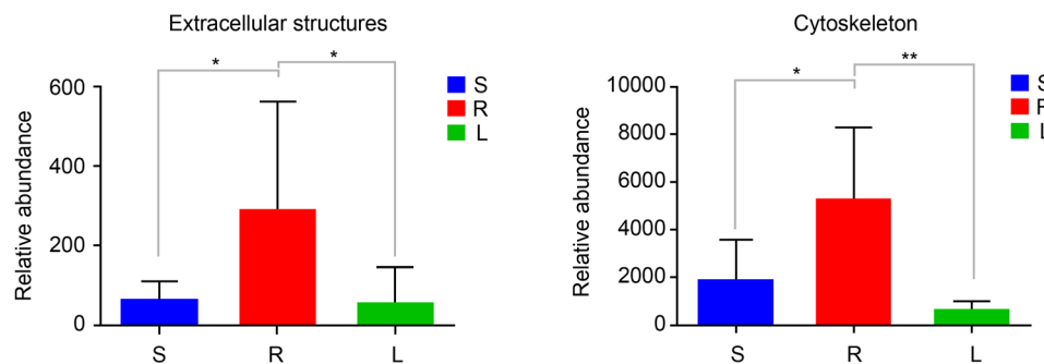
Fig. 8. Significantly relative abundance of roots, stems, and leaves (mean \pm SD) ( n=6 ). A: enriched in extracellular structures. B: enriched in the cytoskeleton. S represents stems, R represents root, and L represents leaf. ( 0.01 < p \leq 0.05 marked as *, 0.001 < p \leq 0.01 marked as **).
