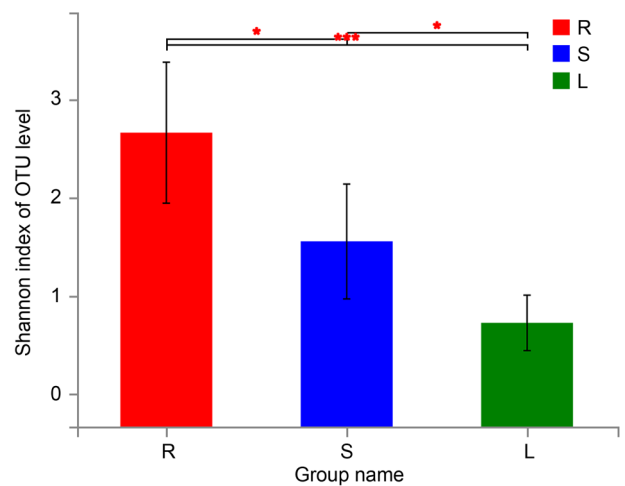
Fig. 3. Shannon index of OTU level of roots, stems, and leaves (mean ± SD) (n = 6). S represents stems, R represents root, and L represents leaf. (0.01 < p ≤ 0.05 marked as *, 0.001 < p ≤ 0.01 marked as **, p ≤ 0.001 marked as ***).
