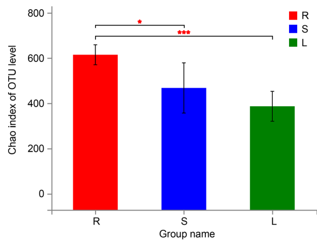
Fig. 2. Chao index of OTU level of roots, stems, and leaves (mean ± SD) (n = 6). S represents stems, R represents root, and L represents leaf. (0.01 < p ≤ 0.05 marked as *, 0.001 < p ≤ 0.01 marked as **, p ≤ 0.001 marked as ***).
