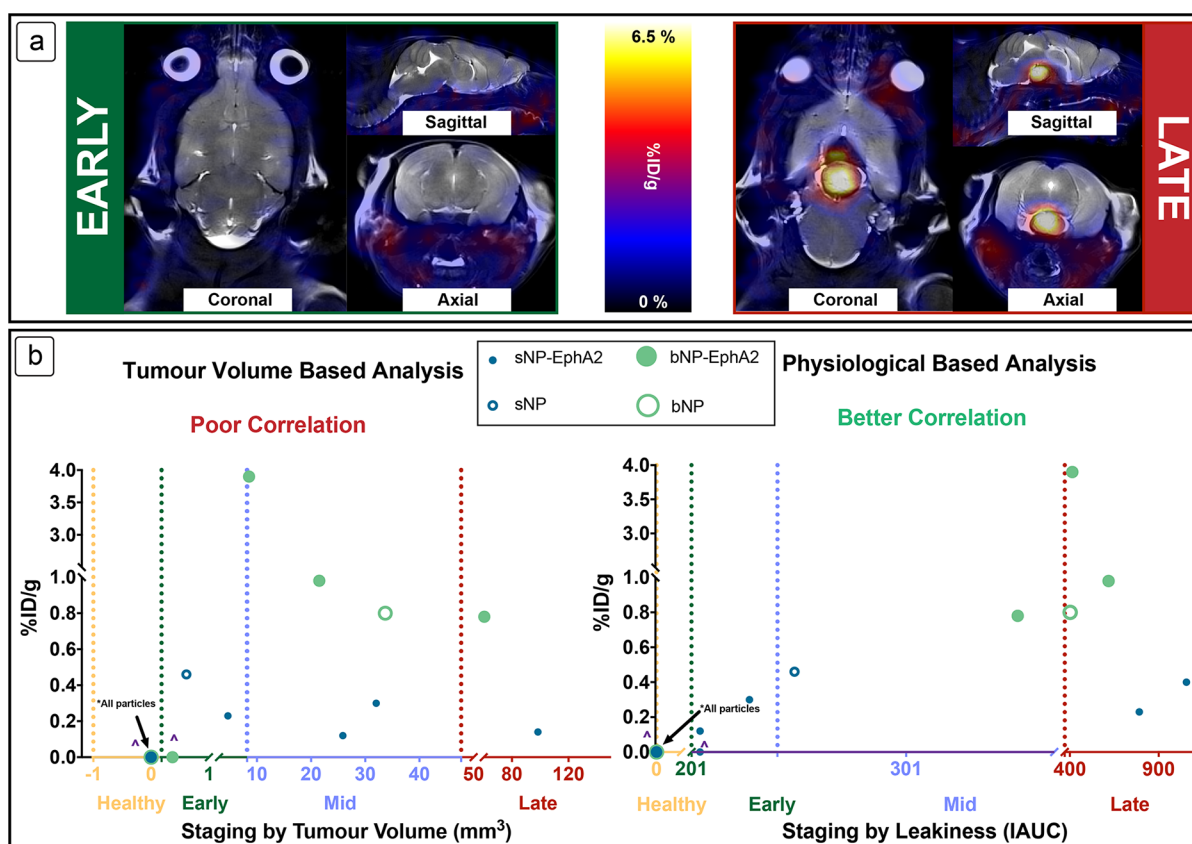
Figure 3. Passage of the nanomedicines across the BBB into the tumor was measured and visualized using PET of 64 Cu labeled sNP and bNP. (a) Representative coronal and sagittal (respectively) images are shown for the early- and late-stage tumors, with the PET signal in red (36 h after injection of radiolabeled nanomedicine), the background MRI in grayscale. (b) Accumulation of 64 Cu labeled nanomedicines as a function of staging by tumor volume or leakiness. Erratic accumulation with no discernible trend is observed when staged by tumor volume, but a clearer picture can be seen when staged by leakiness as measured by Gadovist. \Delta denotes nanomedicines that were injected, but no crossing into the tumor was observed.
