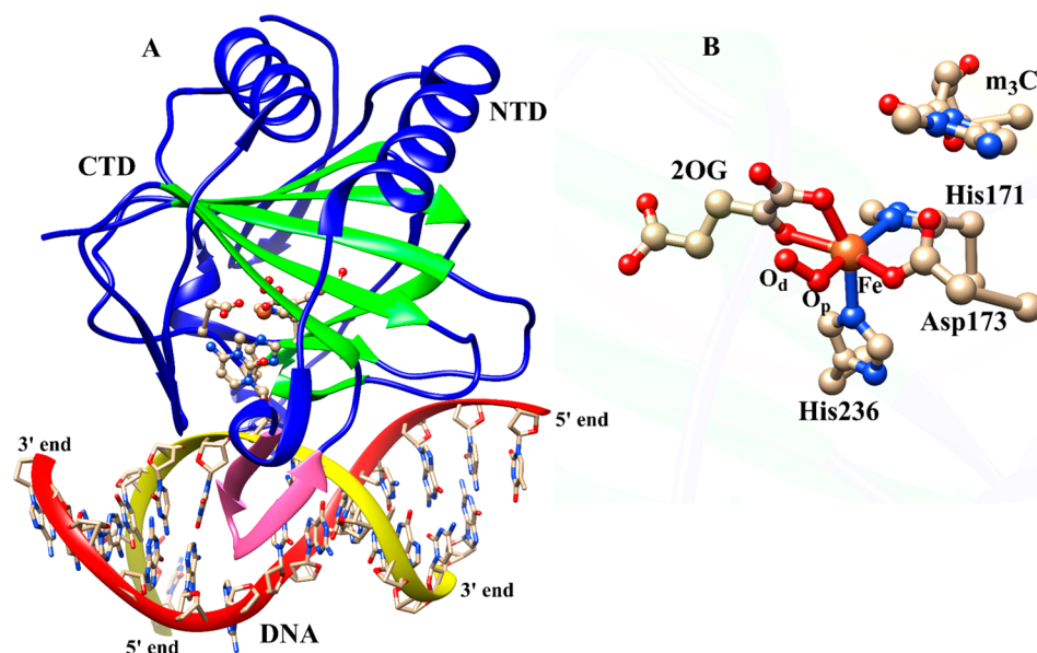
Figure 1. Average structure of AlkBH2–dsDNA (A) and the view of the active site (B) derived from the Fe(III)–superoxo intermediate MD simulations. Coloring: double-stranded beta helix (DSBH) core fold (green) and the hydrophobic \beta -hairpin (pink). NTD and CTD are N-terminal domain and C-terminal domain, respectively.
