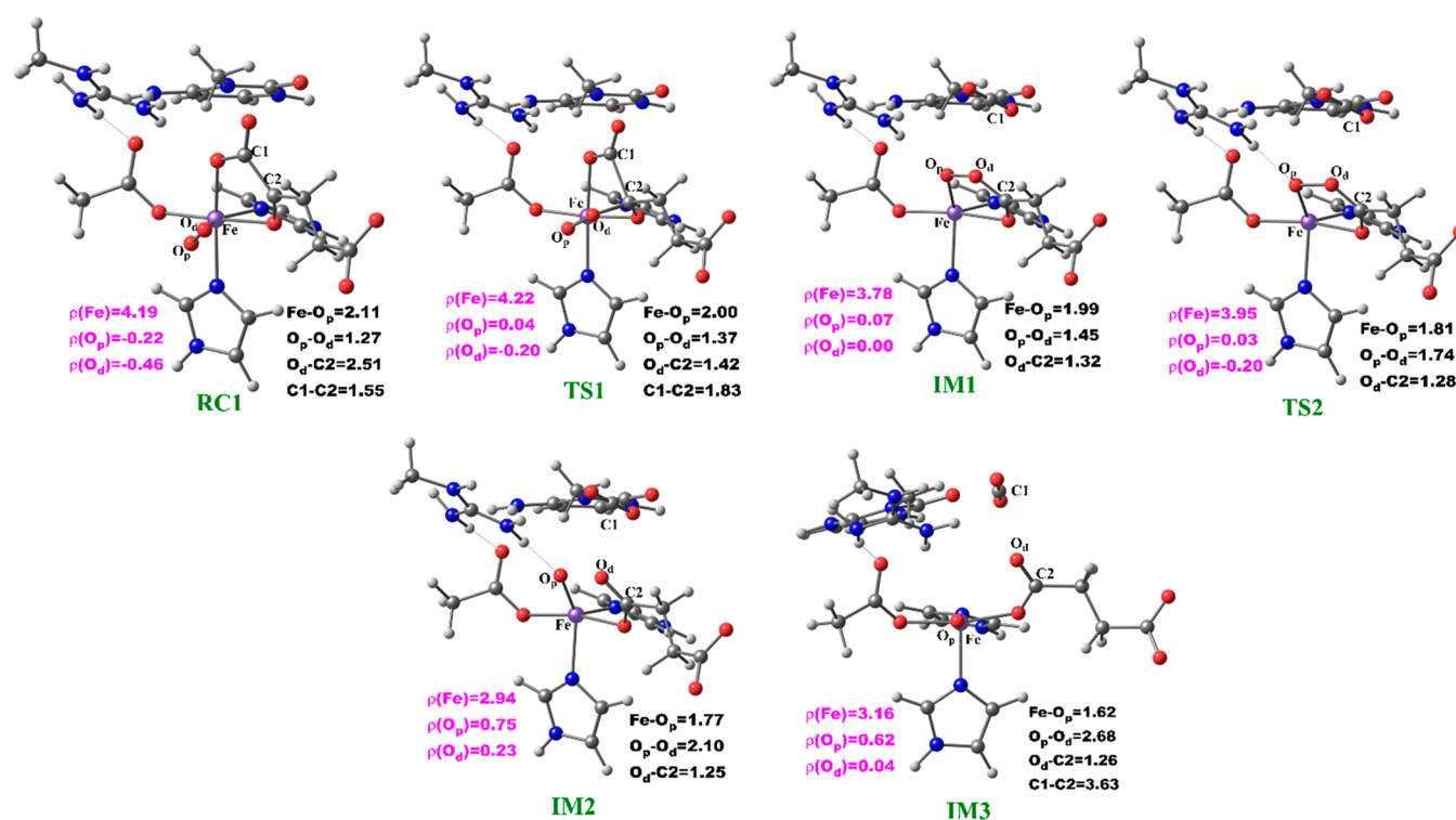
Figure 5. Geometries of the stationary points along the dioxygen activation step in AlkBH2-dsDNA. Distances (Å) and the spin densities are in black and pink, respectively.
