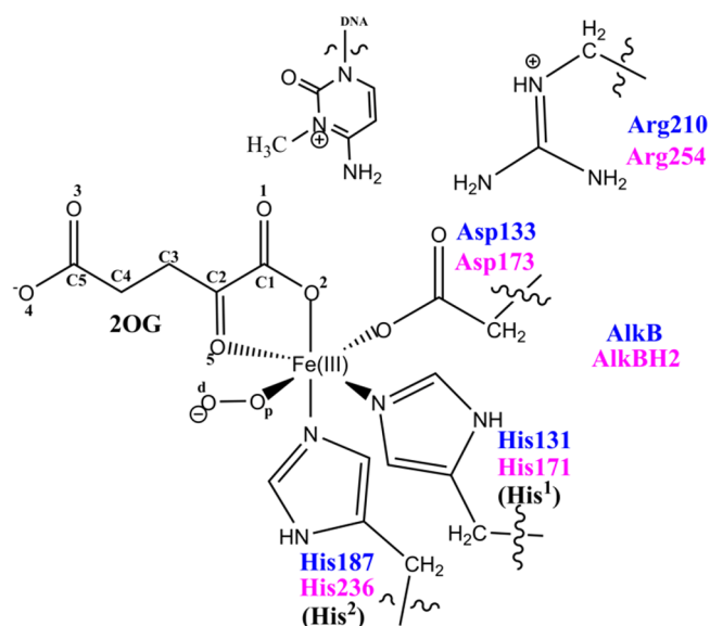
Figure 3. QM region of AlkB/AlkBH2 used in the QM/MM calculations.
