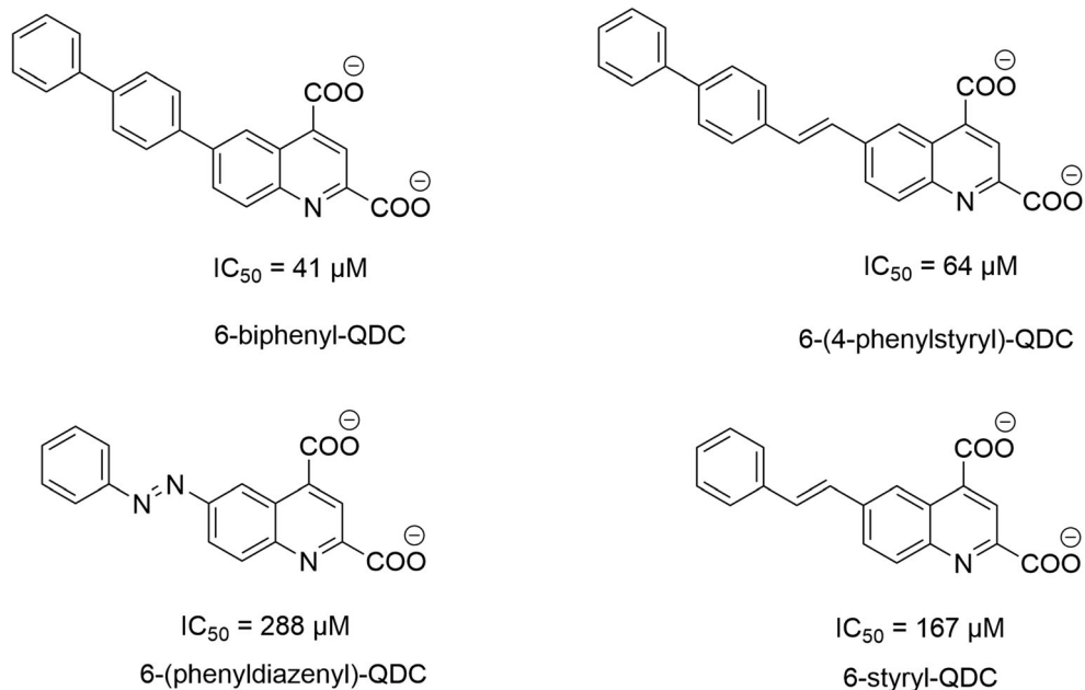
Scheme 4 Structures of QDCs analogs as VGLUTs inhibitors (Carrigan et al., 2002)
