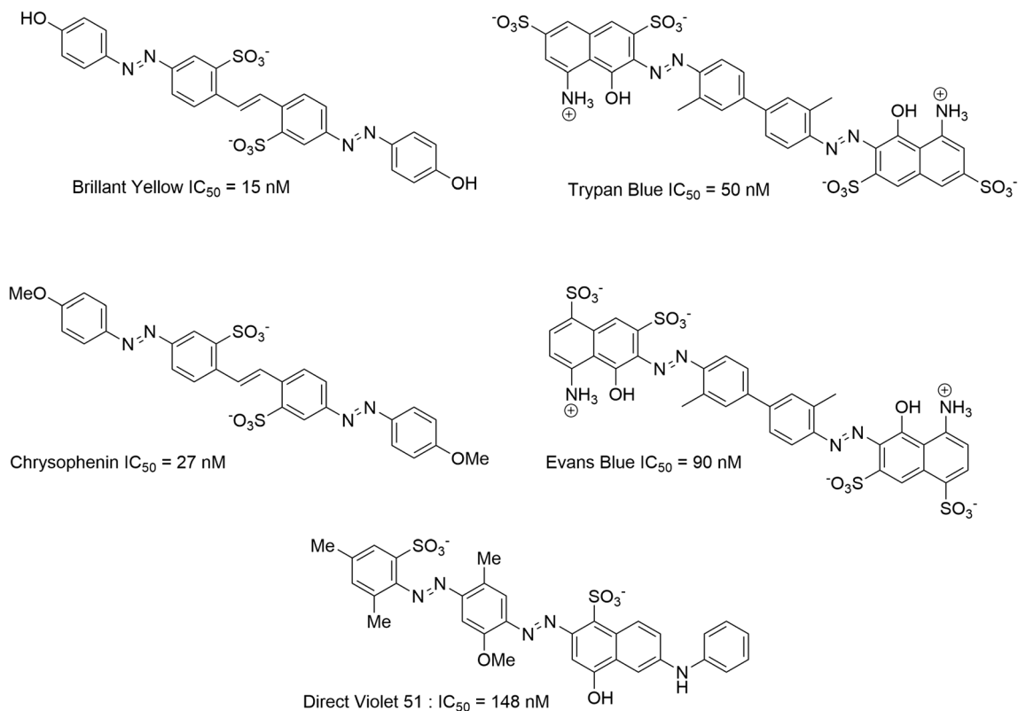
Scheme 5 Azo dyes (Favre-Besse et al., 2014; Omote et al., 2016; Tamura et al., 2013)
