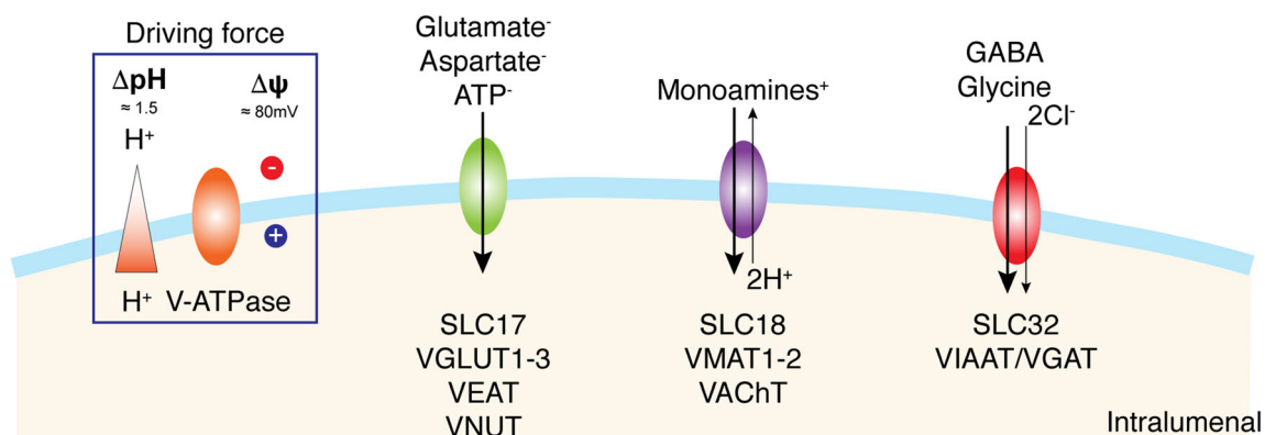
Fig. 1 \text{H}^+ -dependent vesicular neurotransmitter transport. Specific \text{H}^+ -dependent transporters are responsible for neurotransmitter vesicular uptake and belong to different families depending on the global charge of their respective substrates: SLC17 for glutamate and ATP, SLC18 for
