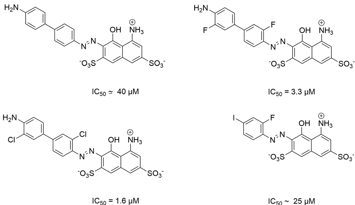
Scheme 6 Importance of the size of azo dyes for VGLUTs inhibition (Favre-Besse et al., 2014)
