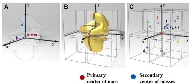
Figure 4. Schematic description of chirality quantifications based on tomographic data for nanoscale structures of arbitrary shape using LH nanoassemblies from Figure 3. (A) Placement of the particle in a Cartesian coordinate system having an origin at the center of total mass. (B) Sectioning NPs with the eight octants of coordinate system (C) Generating the center of mass from eight different partitions.
