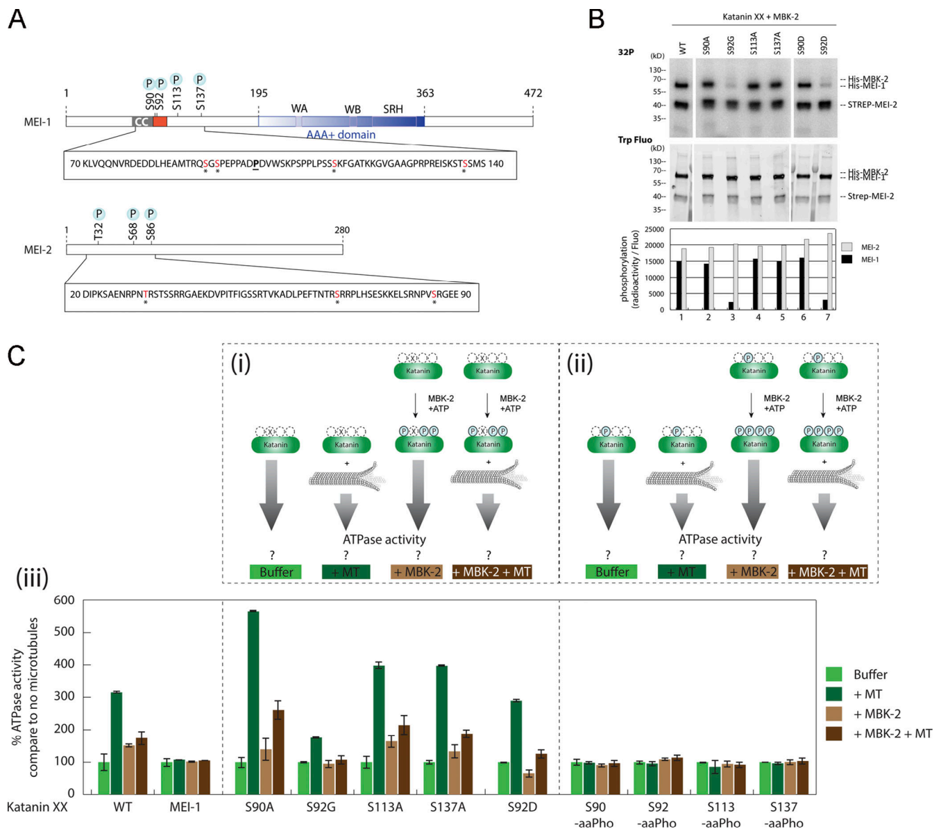
Figure 3. Phosphorylation of the N-terminal disordered region of MEI-1 inhibits the stimulatory effect of MTs on Katanin ATPase activity. (A) Schematic representation of MEI-1 and MEI-2. The positions of phosphorylated sites identified by LC-MS/MS after in vitro phosphorylation of Katanin by MBK-2 are indicated by asterisks (*). Red box represents the PEST sequence, a predicted interacting site for MEL-26 (Fig. S5). AAA+ domain in blue contains Walker A (WA) and Walker B (WB) motifs as well as second region of homology (SRH). CC, coiled-coil. The position of the gain-of-function mutation P99L is indicated (underlined). (B) Radioactive in vitro kinase assays using MBK-2 kinase and Katanin, WT or containing serine to alanine substitutions in MEI-1 N-terminal at specific positions, as substrates. Autoradiograph of SDS-PAGE showing \gamma -[ ^{32} P] incorporation in MEI-1 and MEI-2 (upper panel). Total Katanin present in each lane of the same SDS-PAGE using Stain Free (Bio-Rad), based on tryptophan labeling (middle panel). Gels were quantified using ImageJ, and results are represented in the histogram. The results shown are representative of one experiment that was reproduced three times. (C) Unmodified and phosphorylated Katanin ATPase activity in the absence or presence of MTs. The top panels (Ci and Cii) show the schematics of the experiment and the different Katanin versions used in the assay. Ciii, the bottom panel, shows Katanin ATPase activity presented as percentage of Katanin ATPase activity measured without MTs and without MBK-2. For each Katanin, the measured ATP activity in the absence of MT and MBK-2 was normalized to 100% (first condition, light green bars). (Ci) Katanin (green oval), WT or containing site-specific serine to alanine substitution in MEI-1, was phosphorylated or not by MBK-2, and then the ATPase activity of the enzyme was measured in the absence or presence of MTs. (Cii) Katanin containing MEI-1 phosphorylated at specific sites by genetic code expansion in E. coli was phosphorylated or not by MBK-2, and then the ATPase activity of the enzyme was measured in the absence or presence of MTs. Experiments in each condition were performed at least four times.
