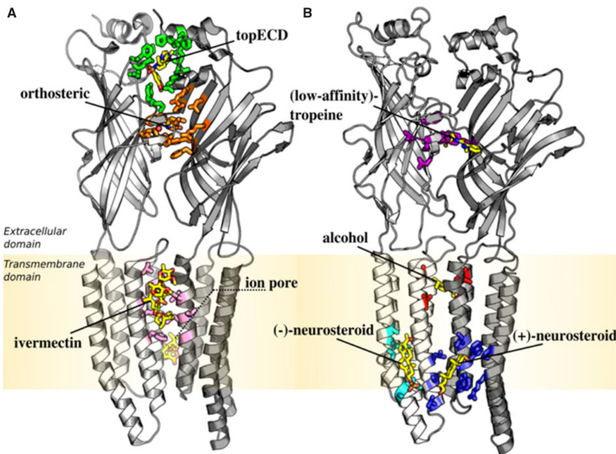
Fig. 2. Topographical location of the actual/putative regulatory sites at GlyR by structural biology. (A) Regulatory sites illuminated by high-resolution structures of GlyR. From top to bottom: (i) the allosteric inter-subunit extracellular site (top-ECD) that accommodates the positive allosteric modulator AM-3607 is shown in green; (ii) the orthosteric site that binds the endogenous neurotransmitter glycine is in orange; (iii) the allosteric inter-subunit site in the transmembrane domain that binds the positive allosteric modulator ivermectin (ivermectin site) is in pink; (iv) the allosteric site for negative modulation by picrotoxin (ion pore site) is in the background. Coordinates for glycine, the allosteric modulators AM-3607 and ivermectin were extracted from the X-ray structure of GlyR- \alpha 3 (PDB: 5VDH; Huang et al. , 2017a). Coordinates for picrotoxin were extracted from the X-ray structure of GABA A R- \alpha 1\beta 3\gamma 2 (PDB: 6HUG; Masiulis et al. , 2019); they are consistent with the most-recent cryo-EM results in GlyR- \alpha 1 (Kumar et al. , 2019). (B) Putative regulatory sites illuminated by high-resolution structures of homologous pLGICs with concordant evidence at GlyR. From top to bottom: (i) the extracellular site for the low-affinity tropeine-binding site is shown in purple with granisetron bound; (ii) the inter-subunit transmembrane site for alcohol binding is in red with propofol bound; (iii) the allosteric intra-subunit binding site for inhibition by neurosteroids or (-)-neurosteroid site is shown in cyan with pregnenolone sulfate (PS) bound; (iv) the allosteric inter-subunit binding site for potentiation by neurosteroids or (+)-neurosteroid site is shown in dark blue with tetrahydrodeoxycorticosterone (THDOC) bound. Coordinates for THDOC and PS were extracted from the X-ray structures of GLIC-GABA A R- \alpha 1 chimera (PDB: 5OSB) and (PDB: 5OSC) (Lavery et al. , 2017), respectively, after structural alignment to GlyR- \alpha 3 in PyMOL (Schrödinger, LLC, 2015). Coordinates for granisetron were extracted from the high-resolution structure of 5-HT 3A receptor (PDB: 6NP0; Basak et al. , 2019). Coordinates for propofol were extracted from the high-resolution structure of GLIC F238A/N239A (PDB: 5MVM; Fourati et al. , 2018). In all cases, residues that are known to be involved in binding of allosteric modulators at GlyR are color-coded
