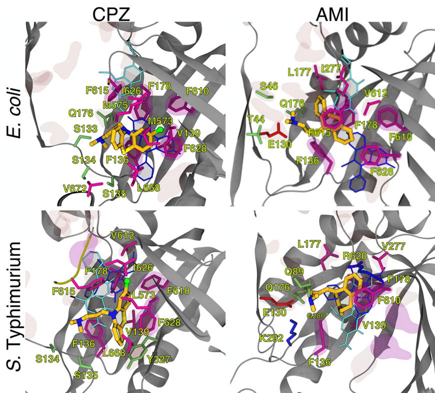
FIG 8 Representative conformations of the most stable binding modes of chlorpromazine and amitriptyline within the DP T of AcrB EC and AcrB ST7 , as obtained from all-atom MD simulations of the periplasmic portion of the transporter in explicit solvent (see Materials and Methods for details and Fig. S3 in the supplemental material). The protein is shown as gray ribbons, the inhibitors as CPK colored by element (C, N, S, and Cl in dark yellow, blue, light yellow, and green, respectively). Side chains of residues within 3.5 Å of the inhibitors are also shown as sticks colored by residue type (hydrophobic, polar, acid, and basic in purple, lime, red, and blue, respectively) and labeled. Side chains of residues defining the DP T and the phenylalanines lining the HT (see Table S1 for the definition of different protein regions) are also shown in transparent red and magenta surfaces, respectively. The most stable conformations of norfloxacin and ethidium bromide as obtained also from all-atom MD simulations are shown for comparison in cyan and blue sticks, respectively.
