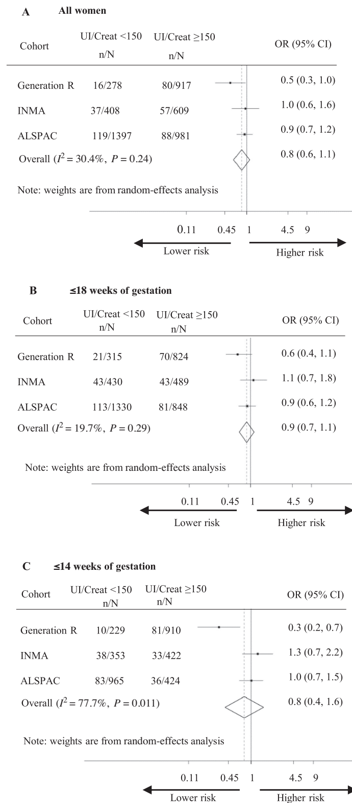
FIGURE 3 Association of maternal UI/Creat <150 \mu\text{g/g} with a high child autistic-trait score \geq 93\text{rd} percentile. Associations depicted as OR (dot) with 95% CI per cohort and overall associations as estimated by random-effects meta-analysis (diamond) in (A) all mother-child pairs, (B) those with \geq 1 measure of UI/Creat at \leq 18 weeks of gestation, and (C) those with \geq 1 measure of UI/Creat at \leq 14 weeks of gestation. Analyses adjusted for maternal age, parity, prepregnancy BMI, smoking during pregnancy, ethnicity/country of birth, maternal educational level, gestational age at urine sampling, child sex, child age, and subcohort in INMA. n = children with a score > 93\text{rd} percentile, N = children with a score < 93\text{rd} percentile. ALSPAC, Avon Longitudinal Study of Parents and Children; INMA, Infancia y Medio Ambiente; UI/Creat, urinary iodine-to-creatinine ratio.
