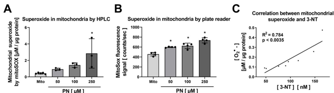
Figure 7. Detection of superoxide generation by mitochondria by mitoSOX HPLC and correlation with 3-NT levels. Isolated heart mitochondria were nitrated by PN at concentrations of 50–250 μM. These samples were split, one aliquot was used for measurement of mitochondrial superoxide formation using mitoSOX/HPLC and the other aliquot for determination of free 3-NT levels by HPLC/ECD after digestion. Mitochondrial superoxide formation was determined using HPLC-based quantification of 2-OH-mito-E+ (A) and ROS formation was measured using a fluorescence plate reader assay for the mitoSOX oxidation products (B). The yield of mitochondrial 3-NT was correlated with superoxide formation rate for the different PN-treated samples (C). HPLC/ECD analysis was performed with 20 μL of sample at 27 °C with isocratic elution (1 mL/min, mobile phase: 26.3 mM sodium citrate and 10.9 mM sodium at pH 3.75 with 3.5 v/v% methanol; 3-NT eluted at 4.05 min). Data are presented as mean ± SD of n = 3–5 (A); n = 4 (B) and n = 8 (C) independent experiments. * indicates p < 0.05 versus Mito untreated control group.
