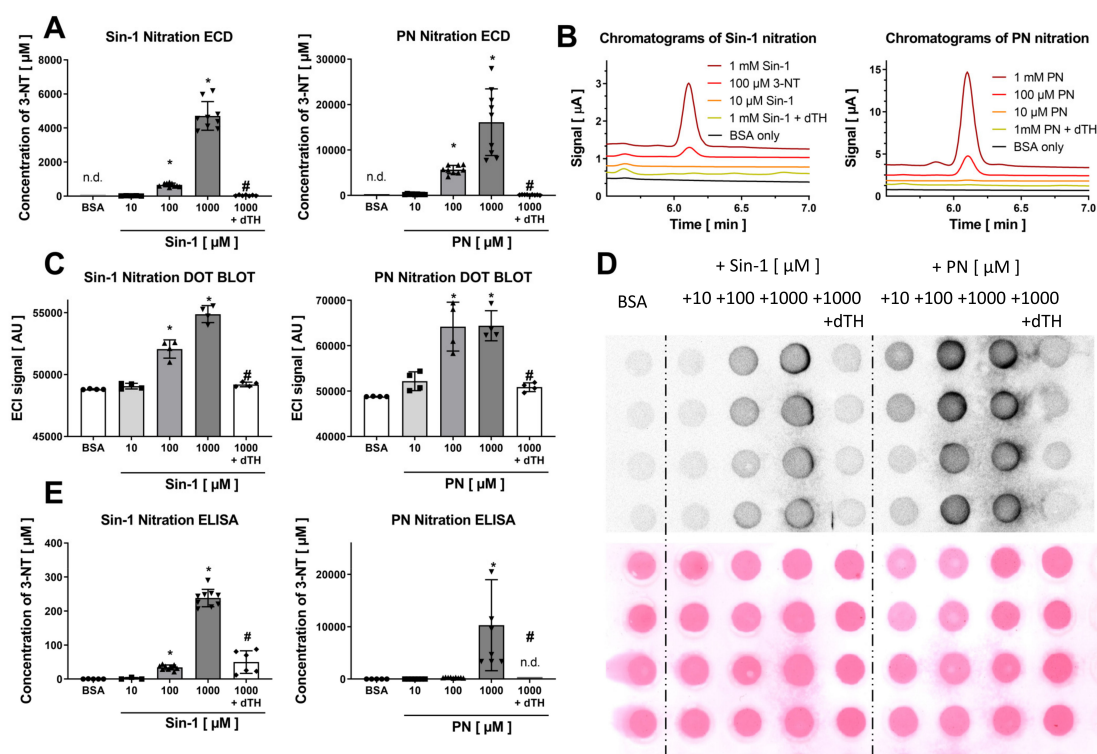
Figure 2. Detection of free 3-NT from nitrated BSA by HPLC/ECD and comparison with detection of BSA-bound 3-NT by antibody-based methods. Purified BSA was nitrated by Sin-1 or PN (10–1000 \mu M) and generated 3-NT was reduced by dTH. These samples were subjected to pronase digest before HPLC/ECD analysis (A) or were not digested for quantification by dot blot (C) and ELISA (E). (B) Representative chromatograms are shown for the HPLC/ECD quantification. (D) Representative blots are shown for the dot blot quantification. Equal protein loading was checked by Ponceau staining of the membrane. HPLC/ECD analysis was performed with 20 \mu L of sample at 27 ^{\circ} C with isocratic elution (1 mL/min, mobile phase: 26.3 mM sodium citrate and 10.9 mM sodium at pH 4.75 with 2.8 v/v % methanol; 3-NT eluted at 6.2 min). Data are presented as mean \pm SD of n = 9 (A), 9 (C) and 4 (E) independent experiments. * indicates p < 0.05 versus BSA untreated control group; # indicates p < 0.05 versus 1000 \mu M Sin-1/PN group.
