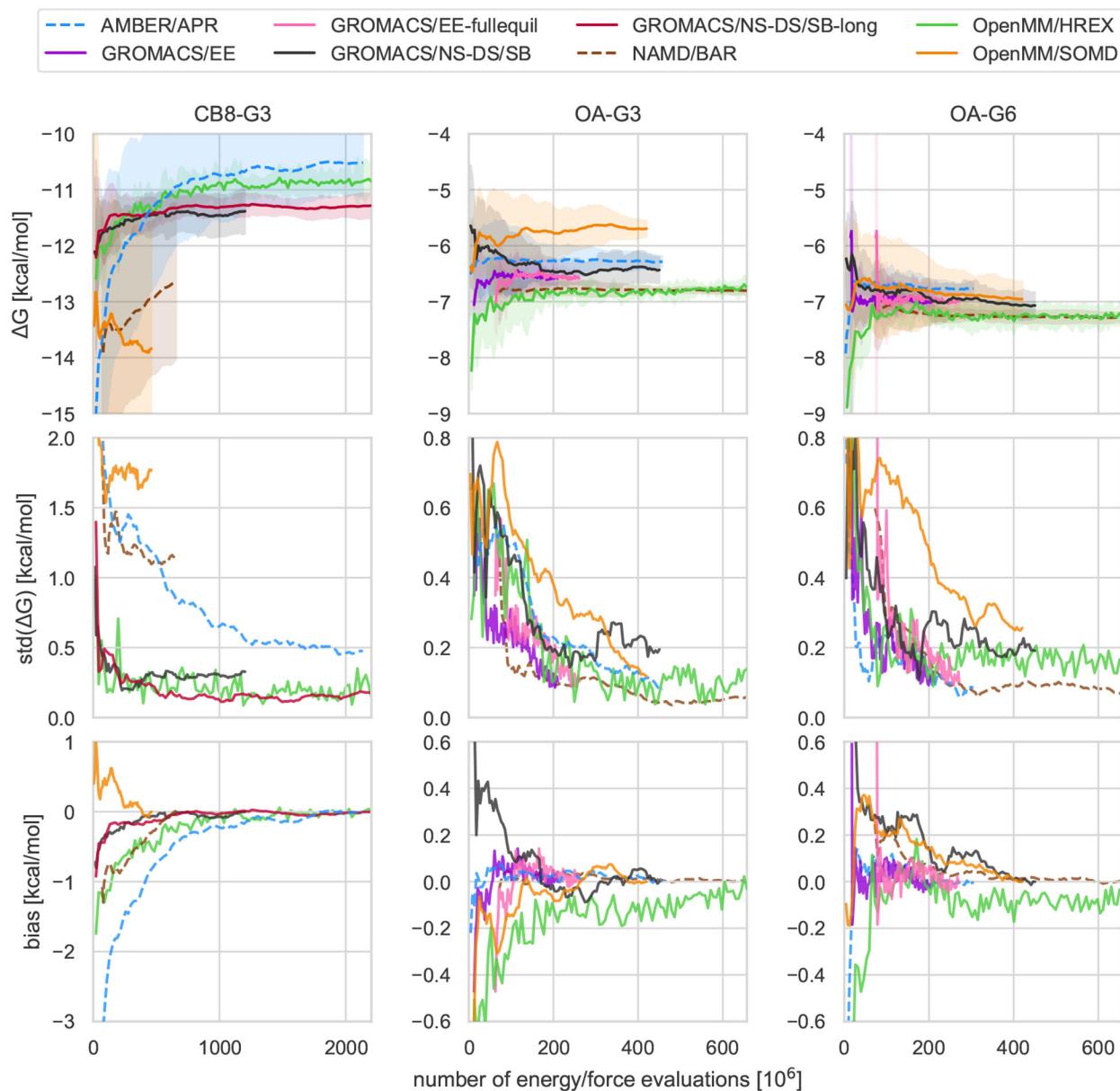
Figure 2. Mean free energy, standard deviation, and bias as a function of computational cost.
