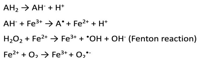
Figure 2. Scheme of hydroxyl radical generation according to Fenton’s predictions. AH_2 —ascorbic acid; AH^- —ascorbate anion; A^\bullet —ascorbyl radical; \bullet OH —hydroxyl radical; O_2^{\bullet -} —superoxide anion.
