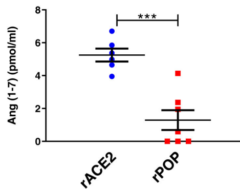
Figure 6: ACE2 and POP proteins in WT sera, lung and kidneys and the effect of rACE2 and rPOP on Ang-(1-7) and Phenylalanine formation.
