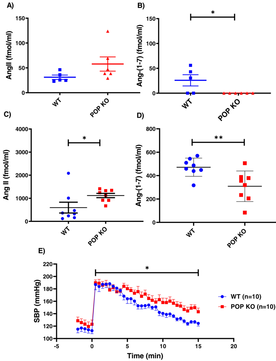
Figure 3: Studies in POPKO mice
