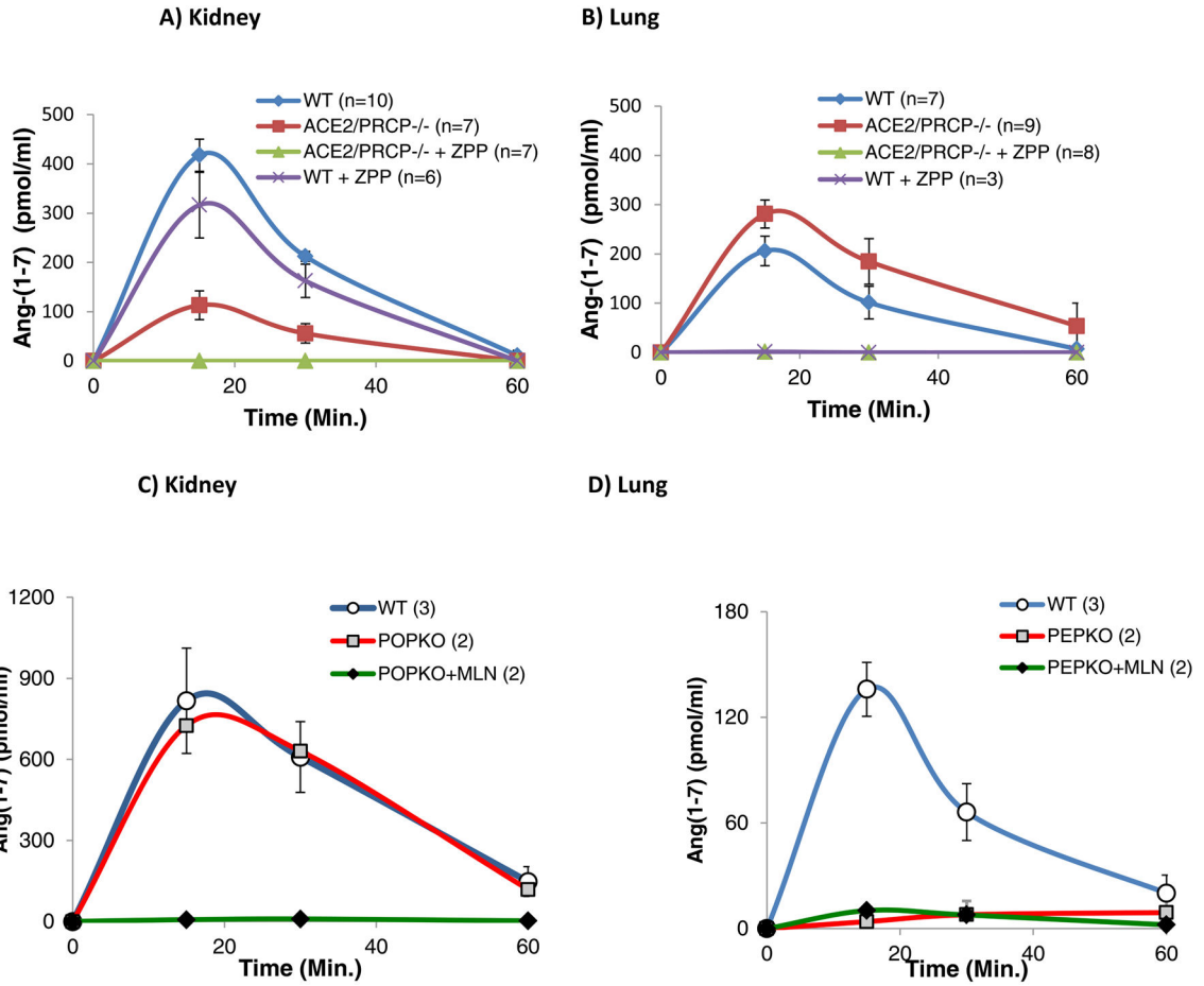
Figure 4: Ex vivo Ang-(1-7) formation from Ang II in kidney and lung lysates as assessed by the peak levels of Ang-(1-7) at 15 minutes (see methods).
