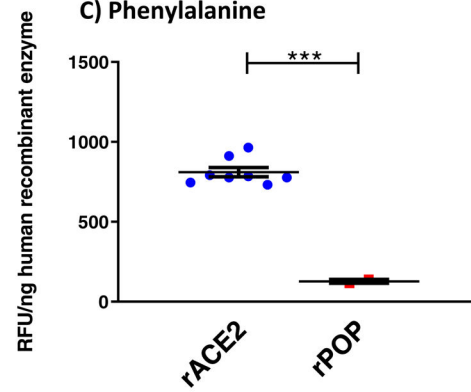
Figure 6: ACE2 and POP proteins in WT sera, lung and kidneys and the effect of rACE2 and rPOP on Ang-(1-7) and Phenylalanine formation.
