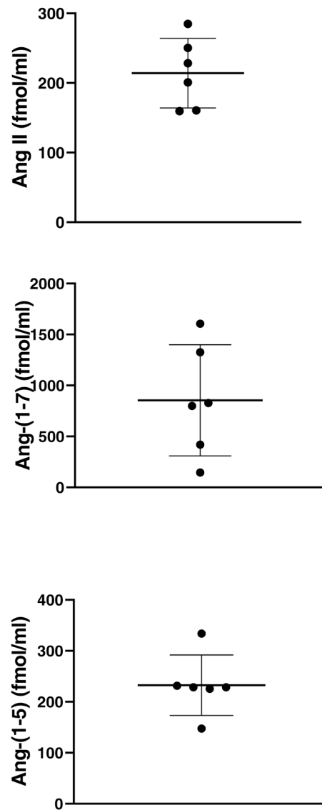
Figure 1: Angiotensin peptide levels in serum measured by LC/MS-MS in Ang II-infused mice. Plasma showed high levels of Ang II (upper), Ang-(1-7) (middle), and Ang-(1-5) (lower panel) measured by Liquid Chromatography Tandem Mass Spectrometry (LC/MS-MS). Blood was obtained by cardiac puncture from mice (n=6) at 5 minutes after Ang II i.p. infusion.
