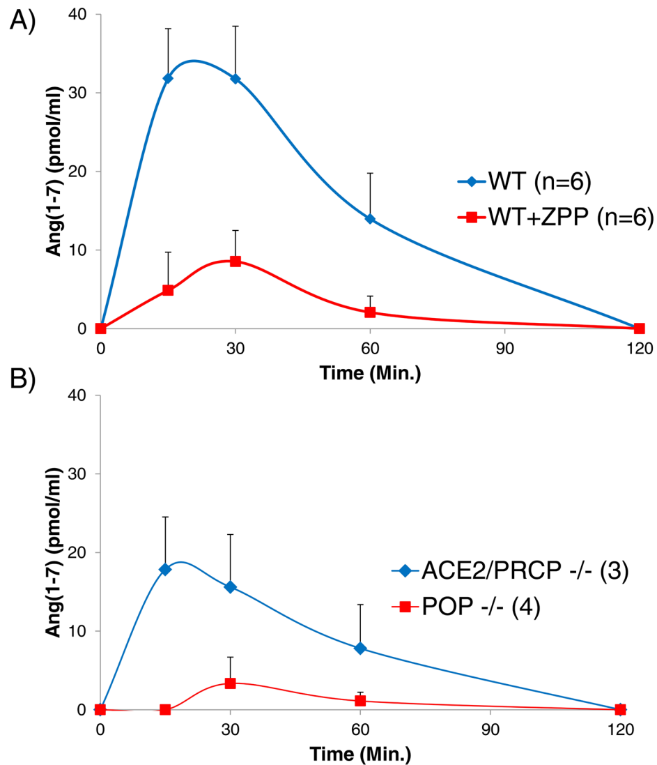
Figure 5: Ex vivo formation of Ang-(1-7) from Ang II in serum.
