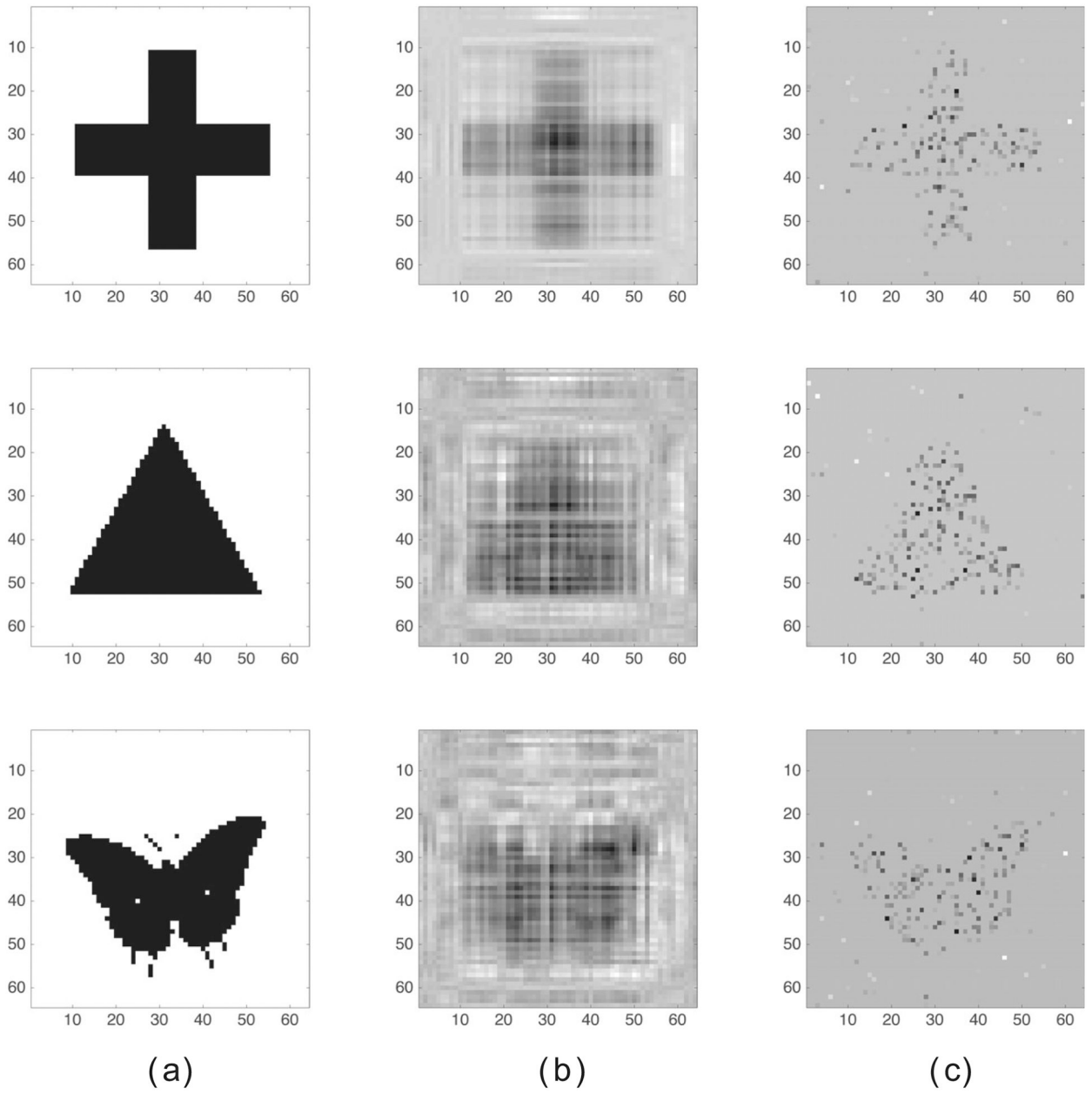
Figure 1. The figures for cross image: (a) original signal; (b) our nuclear regularization estimate; and (c) l_1 -regularized estimate.
