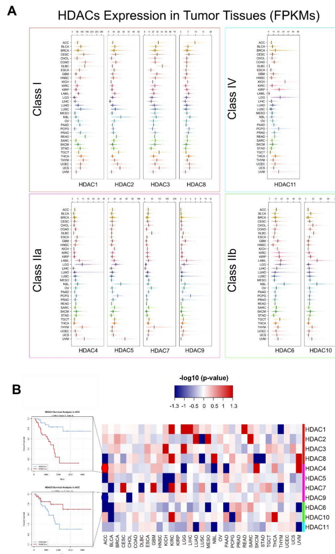
Figure 6. (A) Transcript levels of HDACs 1–11 in tumor tissues expressed in FPKM. Boxplots shows the expression of Class I (red box), Class IIa (pink box), Class IIb (green box), and Class IV (aquamarine box) from tumor samples in the pan-cancer TCGA dataset [187]. Tumor types are: ACC, adrenocortical carcinoma; BLCA, bladder urothelial carcinoma; BRCA, breast invasive carcinoma; CESC, cervical squamous cell carcinoma and endocervical adenocarcinoma; CHOL, cholangiocarcinoma; COAD, colon adenocarcinoma; DLBC, lymphoid neoplasm diffuse large B-cell lymphoma; ESCA, esophageal carcinoma; GBM, glioblastoma multiforme; HNSC, head and neck squamous cell carcinoma; KICH, kidney chromophobe; KIRC, kidney renal clear cell carcinoma; KIRP, kidney renal papillary cell carcinoma; LAML, acute myeloid leukemia; LGG, brain lower grade glioma; LIHC, liver hepatocellular carcinoma; LUAD, lung adenocarcinoma; LUSC, lung squamous cell carcinoma; MESO, mesothelioma; OV, ovarian serous cystadenocarcinoma; NBL, TARGET-neuroblastoma [188]; PAAD, pancreatic adenocarcinoma; PCPG, pheochromocytoma and paraganglioma; PRAD, prostate adenocarcinoma; READ, rectum adenocarcinoma; SARC, sarcoma; SKCM, skin cutaneous melanoma; STAD, stomach adenocarcinoma; TGCT, testicular germ cell tumors; THYM, thymoma; THCA, thyroid carcinoma; UCS, uterine carcinosarcoma; UCEC, uterine corpus endometrial carcinoma, UVM, uveal melanoma. Expression was FPKM-normalized using the length of ENSEMBL longest isoform and RNA-Seq data from TCGA. (B) Integrated HDAC survival analysis across tumors. Color intensity in the heatmap is proportional to -\log_{10}(p\text{-value}) , a threshold of 1.3 corresponds to a p\text{-value} = 0.05 . Red boxes in the heatmap correspond to a worse OS when the corresponding HDAC is upregulated, while blue boxes mean a better OS in case of upregulation, as shown by example survival curves (left side).
