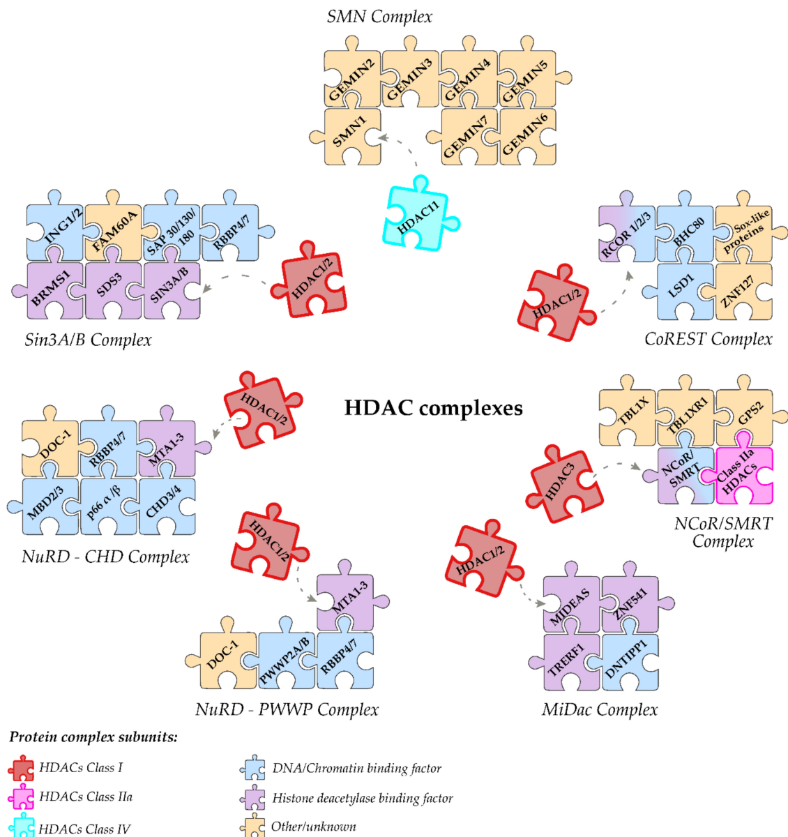
Figure 5. Schematic representation of the well characterized human HDAC-containing core complexes. Color schemes associated with HDACs subunits refer to sequence-based classification of HDACs described in this review. The recruitment of each HDAC in the core complex is depicted schematically with grey arrows that also identifying the HDAC-binding subunit. The HDAC1/2/11-binding subunit within each complex is indicated by the purple color. In addition, each complex contains multiple DNA/chromatin binding subunits indicated in blue. Finally, other subunits, where the biological function in each complex is still uncharacterized, are indicated by the sandy color. The puzzle piece representation and orientation does not reflect specific surface interaction regions. HDAC1/2 indicates 1 or 2, interchangeably (not as a heterodimer).
