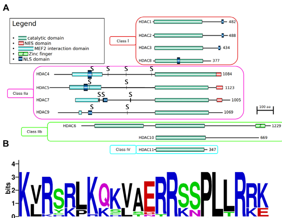
Figure 2. (A) Domain architecture of HDAC proteins (human HDACs are used as reference). S indicate Serine residuals phosphorylated by CaM kinases [41]. (B) Sequence logo of Class IIa HDAC NLS sequence across human, mouse, chicken, and zebrafish proteins. Amino acid coloring indicates their predominant chemical property (blue: basic; red: acidic; green: polar; black: hydrophobic; purple: neutral). Logo generated with WebLogo [49].
