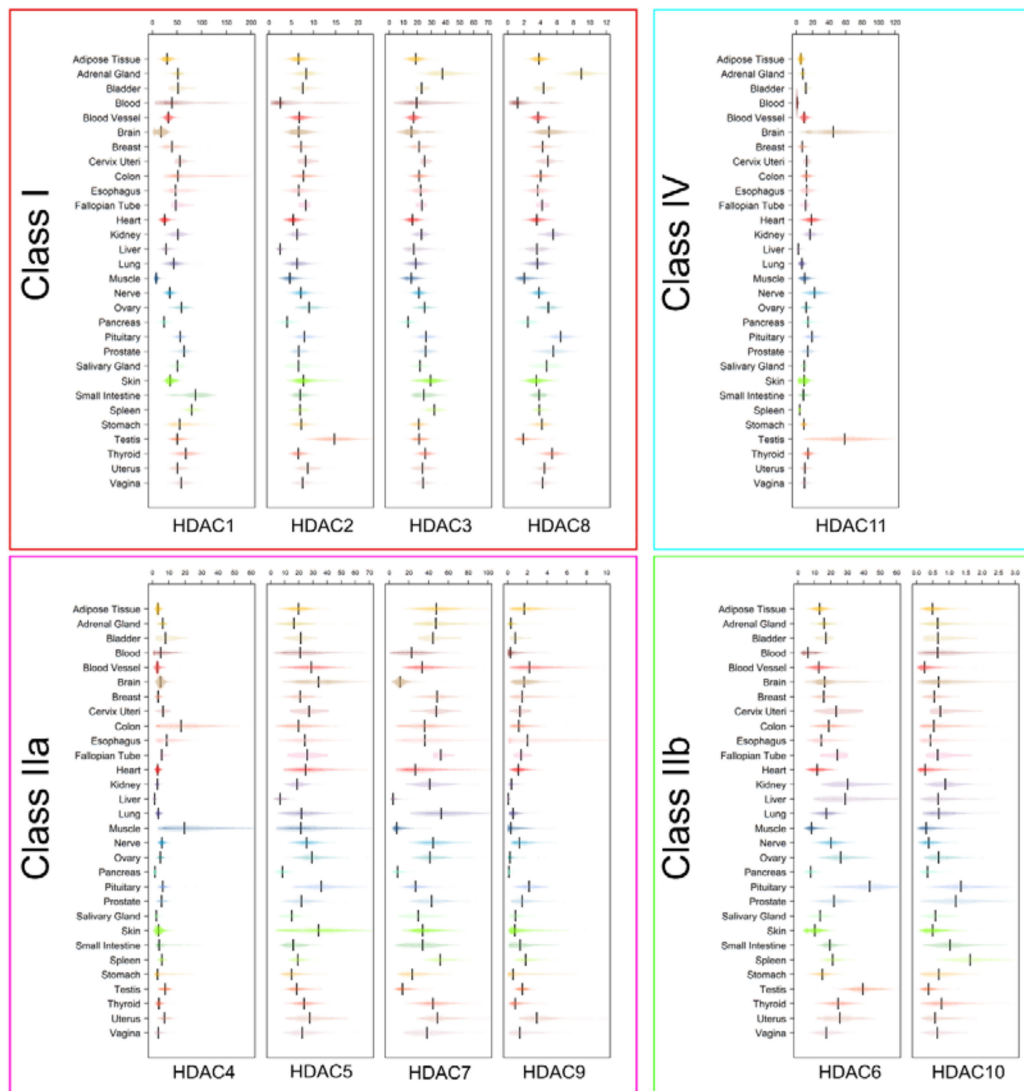
Figure 4. Transcript levels of HDACs 1–11 in healthy tissues expressed in FPKM (fragments per kilobase of transcript length per million of mapped reads). Boxplots show the expression of Class I (red box), Class IIa (pink box), Class IIb (green box), and Class IV (aquamarine box) from normal samples in the GTEx Release V8 dataset. Expression was FPKM-normalized using the length of ENSEMBL longest isoform and RNA-Seq data from GTEx [105].
