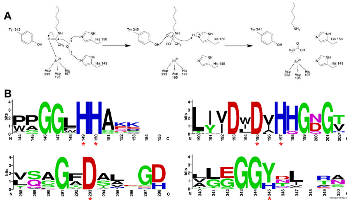
Figure 3. Catalytic action of HDACs. (A) Proposed mechanism of acetyl-lysine hydrolysis catalyzed by HDACs. (B) Sequence conservation of four regions containing the key catalytic amino acids (red asterisks) between all HDACs of the model species used for the phylogenetic tree in Figure 1. Residue Y345 is replaced by an H only in vertebrate Class IIa HDACs.
