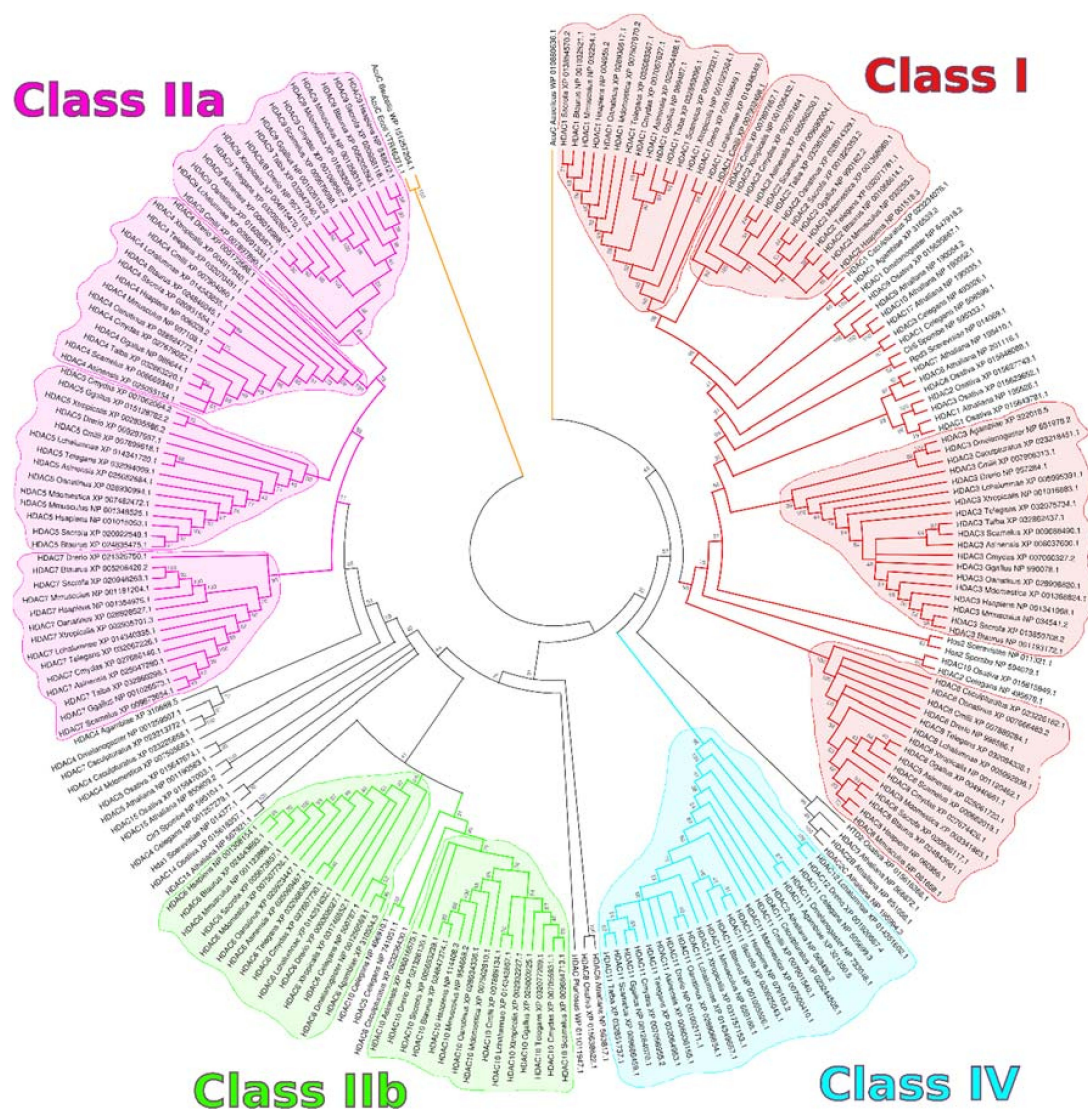
Figure 1. Topological phylogenetic tree representation of 226 representatives of the HDAC protein family. The longest RefSeq protein isoform was selected for each separate gene locus. Multiple sequence alignment was performed using the MUSCLE algorithm [32]. Evolutionary distances were computed as the number of amino acid substitutions per site using the Poisson correction method [33]. The implementation of these algorithms and the visualization were achieved through MEGA X [34]. All 226 sequences used for the generation of this figure are available as Supplementary File S2, in FASTA format. Coloring of branches indicate the putative HDAC class: red for Class I, magenta for Class Ia, green for Class IIb, and cyan for Class IV. Colored areas delimit clades associated to each one of the 11 human HDACs.
