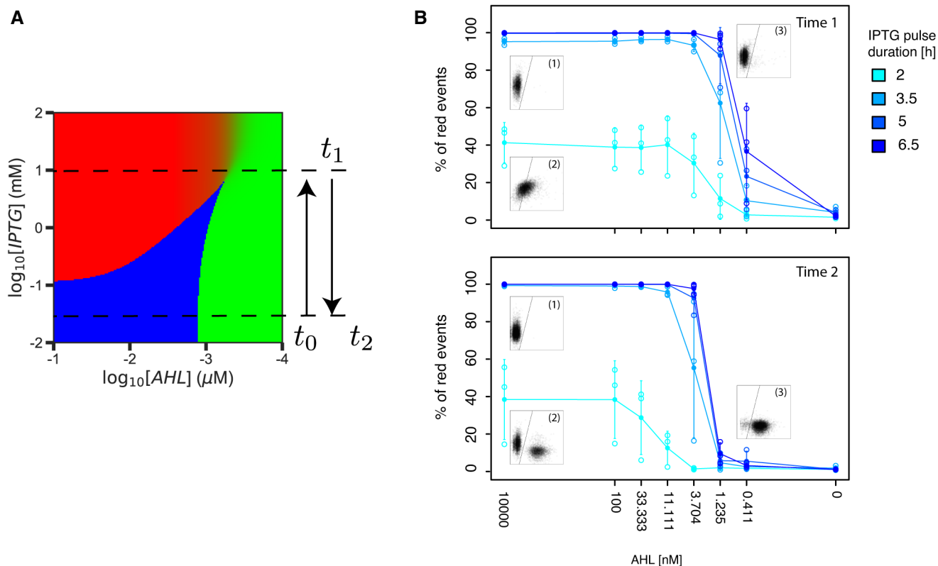
Figure 5. A homogeneous pulse of IPTG allows to control the pattern formation.
