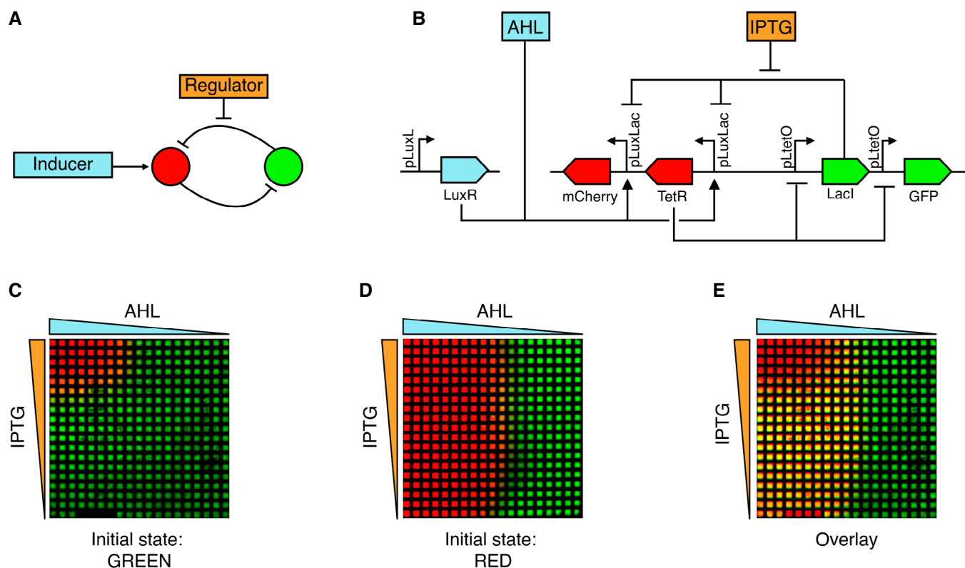
Figure 1. Inducible toggle switch topology and its spatial patterning behavior.
