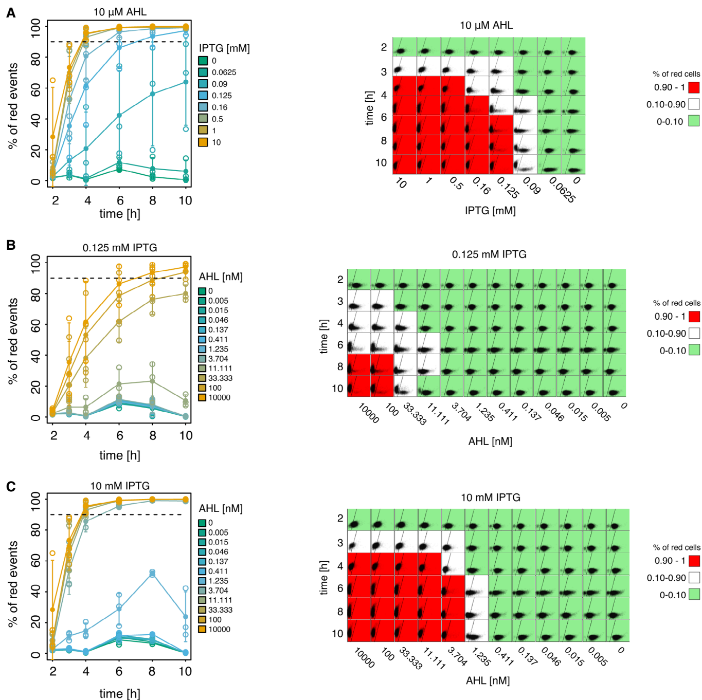
Figure 3. Temporal dynamics of patterning with the inducible toggle switch.
