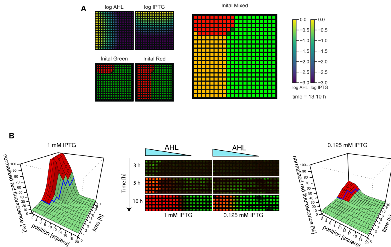
Figure 4. Patterning in the sigmoidal regime is faster than that in the bistable regime.
