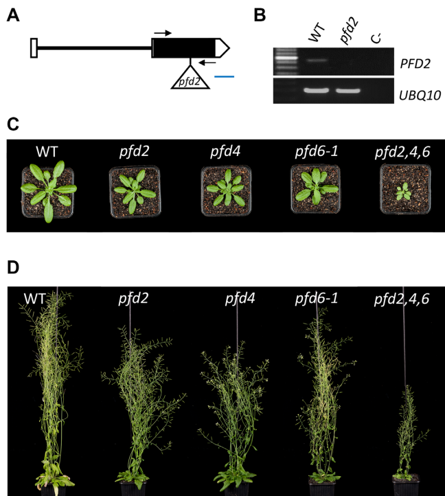
Figure 3. Characterization of novel pfd mutants. (A, B) The novel pfd mutant is a null allele. (A) Structure of the PFD2 gene indicating the position of the insertion. Boxes and line indicate exons and intron, respectively. Open boxes correspond to the 5' and 3' untranslated regions. The triangle indicates the Ds element insertion. Arrows indicate the position of the primers used for the semi-quantitative RT-PCR. Blue line represents 100 bp. (B) Semi-quantitative RT-PCR analysis of PFD2 expression in WT and mutant plants and the negative control (C-; water). The expression of UBQ10 , a housekeeping gene, was used as control. (C) Rosette of 29-d-old plants of the indicated phenotypes at bolting. (D) Global morphological phenotype of 58-day-old plants of the indicated genotypes.
