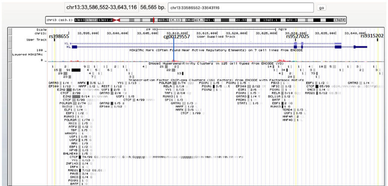
Figure 1. The figure shows the region of the KL gene, including the three SNPs that were evaluated (yellow lines labeled by rs #), cg00129557, and the DNase hypersensitivity site just below this DNAm locus (as indicated by the vertical blue line). The figure was generated using the University of California, Santa Cruz (UCSC) Genome Browser (Kent et al., 2002).
