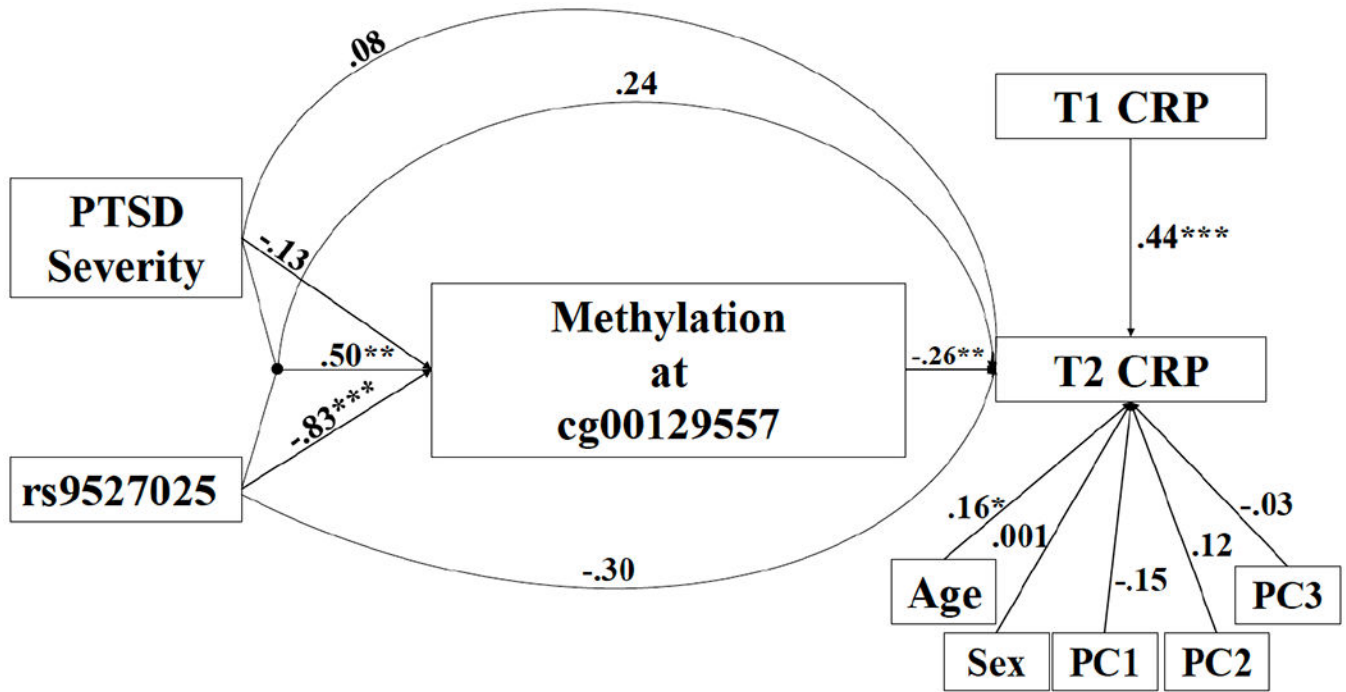
Figure 3. The figure shows the results of the path model examining the direct and indirect effects of the KL-VS SNP (rs9527025), PTSD severity, and their interaction on residualized changes in CRP levels over the course of approximately two years via methylation at the KL locus cg00129557 ( n = 111 ). Standardized coefficients are presented. *p < .05 . **p < .01 . ***p < .001
