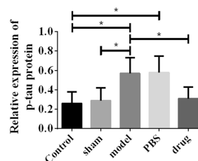
Figure 2 Nimodipine affected CI after SAH through the lncRNA NEAT1/miR-27a/MAPT axis. (A) The binding site (marked in red) of miR-27a to lncRNA NEAT1 and MAPT; (B) the binding site verified by DLR gene assay; (C) effects of nimodipine on lncRNA NEAT1; (D) effects of nimodipine on miR-27a; (E) effects of nimodipine on MAPT and tau protein; *indicated P<0.05, **indicated P<0.01, and ***indicated P<0.001.
