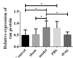
Figure 2 Nimodipine affected CI after SAH through the lncRNA NEAT1/miR-27a/MAPT axis. (A) The binding site (marked in red) of miR-27a to lncRNA NEAT1 and MAPT; (B) the binding site verified by DLR gene assay; (C) effects of nimodipine on lncRNA NEAT1; (D) effects of nimodipine on miR-27a; (E) effects of nimodipine on MAPT and tau protein; *indicated P<0.05, **indicated P<0.01, and ***indicated P<0.001.
