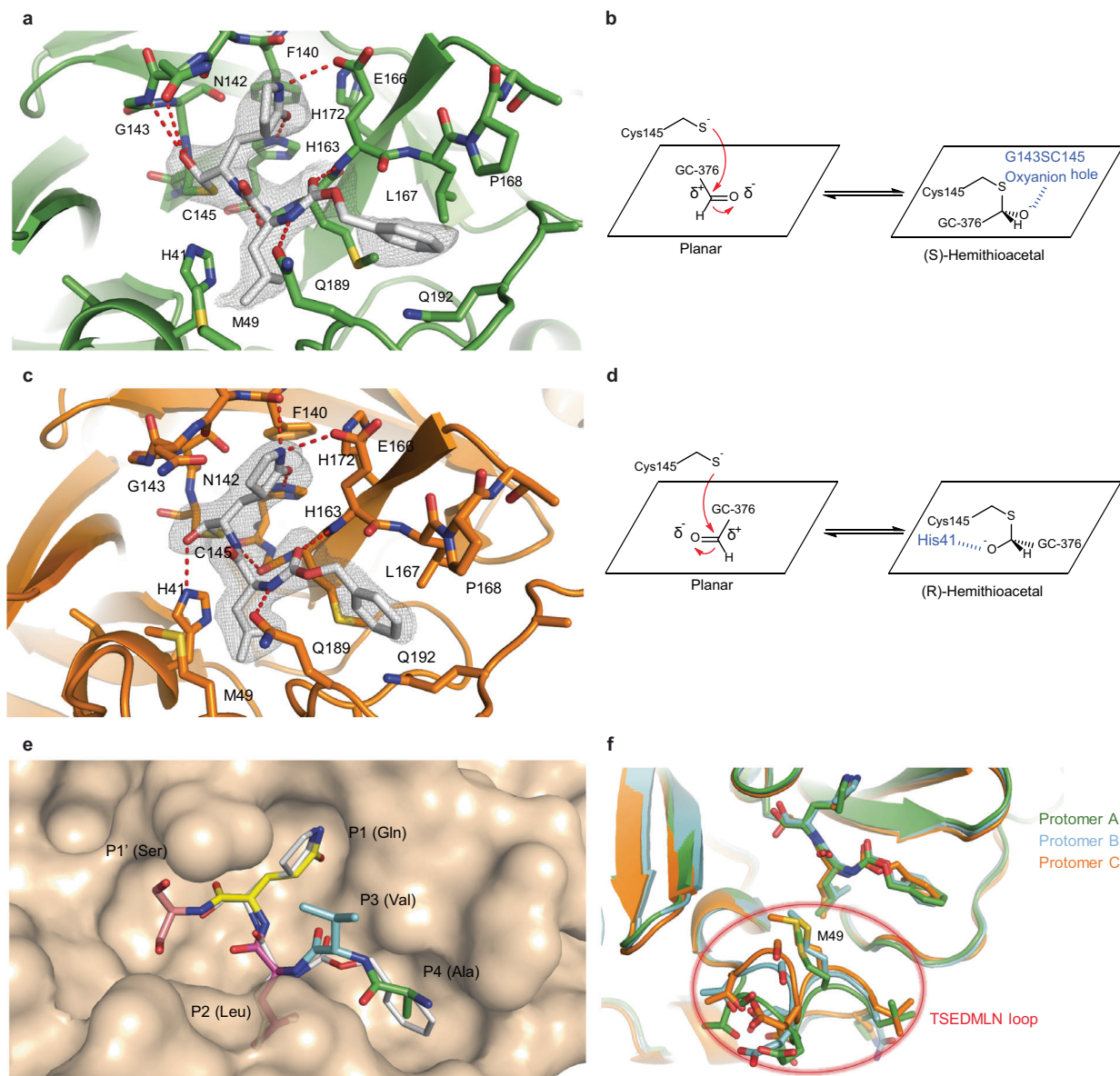
Fig. 6 Molecular recognition of GC-376 ( 64 ) by SARS-CoV-2 M Pro . Complex of SARS-CoV-2 M Pro and GC-376 ( 64 ) with protomer A ( a , b ) and protomer C ( c , d ). Unbiased F_o - F_c map, shown in gray, is contoured at 2\sigma . Hydrogen bonds are shown as red dashed lines. e Surface representation of SARS-CoV-2 M Pro + GC-376 ( 64 ) (white) superimposed with the SARS-CoV M Pro natural, N-terminal substrate (PDB ID: 2Q6G, with residues P1'–P4 in different colors). The SARS-CoV-2 M Pro cleaves between the P1' and P1 residues. f Superimposition of the three protomers in the asymmetric subunit of SARS-CoV-2 M Pro with GC-376 ( 64 ). Significant conformational flexibility is observed, particularly in the TSEDMLN loop.
