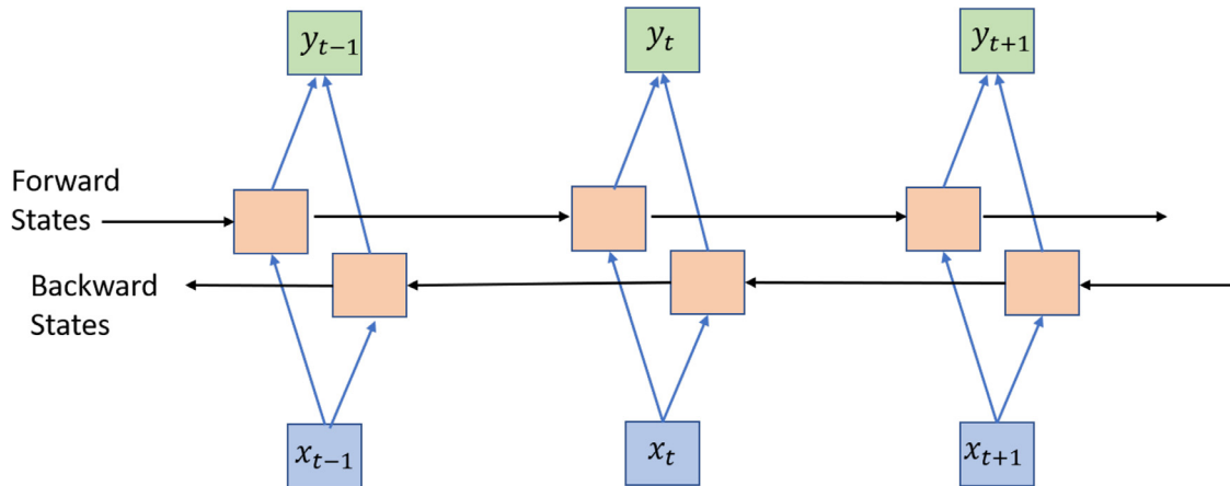
Fig. 4. Bidirectional LSTM.
