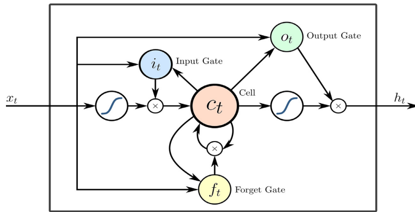
Fig. 1. LSTM Cell.
