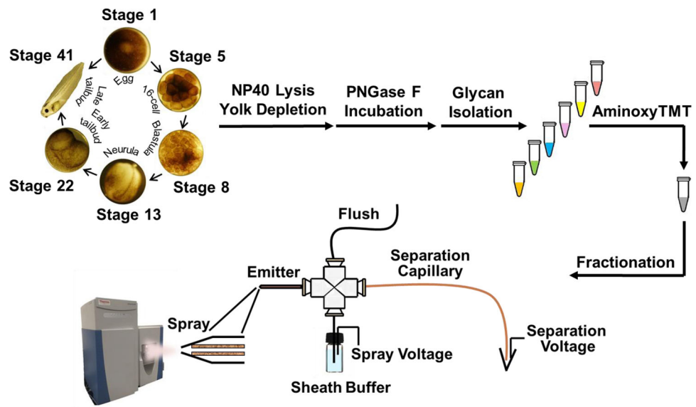
Fig. 1. Analytical pathway of multiplexing N-glycomics quantitation of Xenopus laevis embryogenesis using custom-built CZE-ESI-MS/MS platform with a third-generation electrokinetically-pumped sheath-flow nanospray interface.
