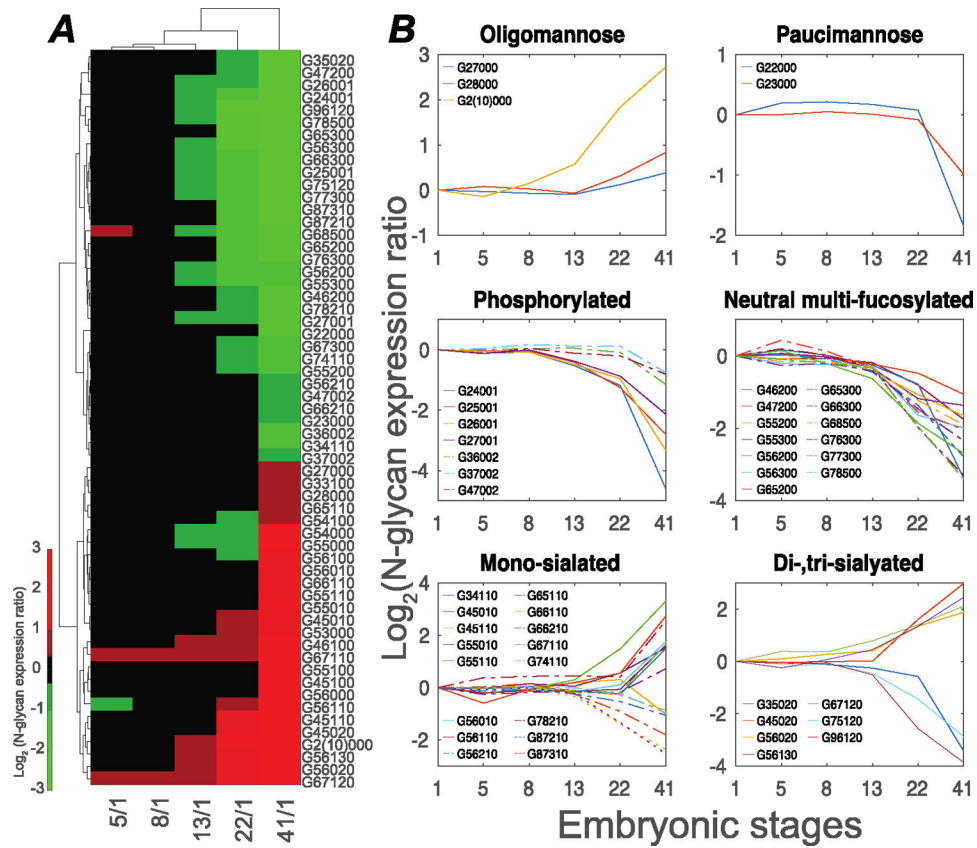
Fig. 4. Xenopus laevis embryo N-glycome analysis. A) Heatmap displaying variations of statistically significant ( p -value<0.027) N-glycan compositions expressed at stage 41. B) Structural clustering of quantified N-glycans with statistically significant changes across six embryonic time points.
