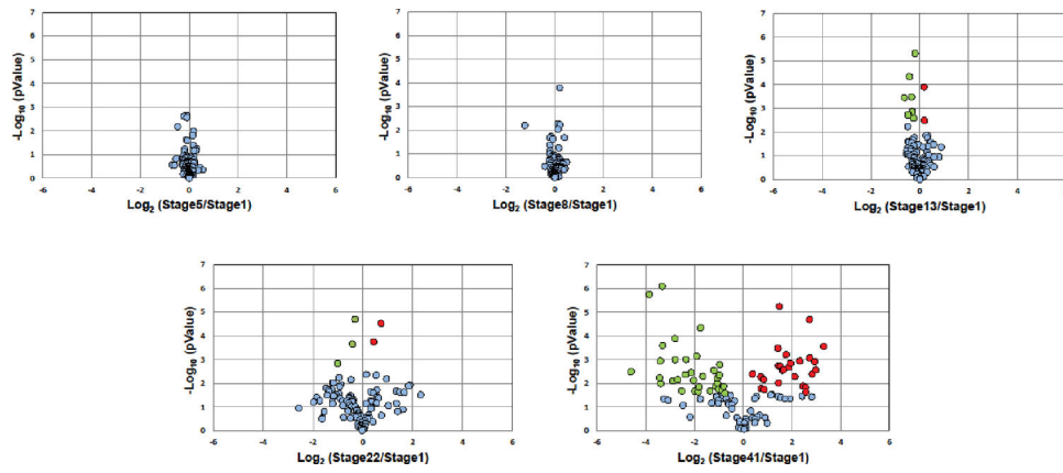
Fig. 3. Volcano plots of the quantified N-glycan compositions over six embryonic stages during development. Glycans with significant changes are marked in red (increase) and green (decrease), respectively.
