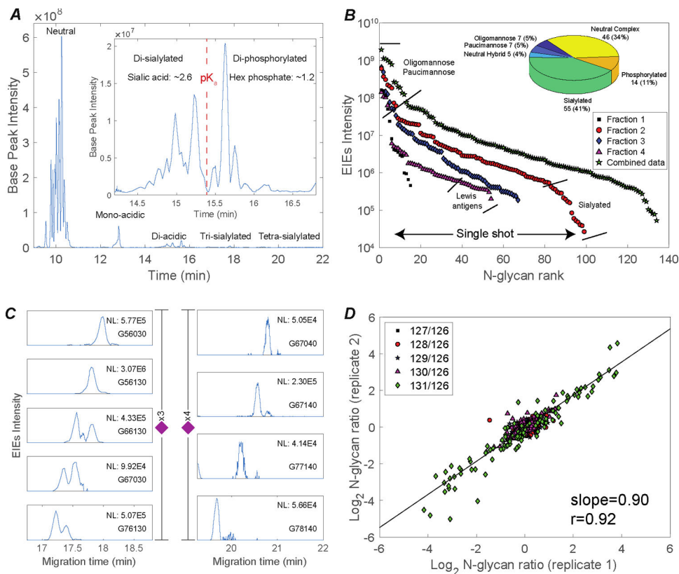
Fig. 2. Deep N-glycome discovery and quantitation of sixplexed sample using CZE-ESI-MS/MS. A) Base peak electropherogram of fraction 2 (red circles in panel B); inset shows the resolution of di-sialylated and di-phosphorylated species. B) N-glycan abundances covering 3–4 orders of magnitude dynamic range in single-shot CZE-ESI-MS/MS analysis of the four fractions, and spanning a 4 orders of magnitude concentration range in the concentration-adjusted combined data. The inset shows the numbers of identified glycan compositions. C) Extracted ion electropherograms (EIEs) of low abundance tri- and tetra-sialylated N-glycans. Glycan compositions are represented as G (HexNAc; Hex; Fuc; NeuAc; phosphate). D) Galaxy plot correlating N-glycan changes in abundance between the two technical replicates.
