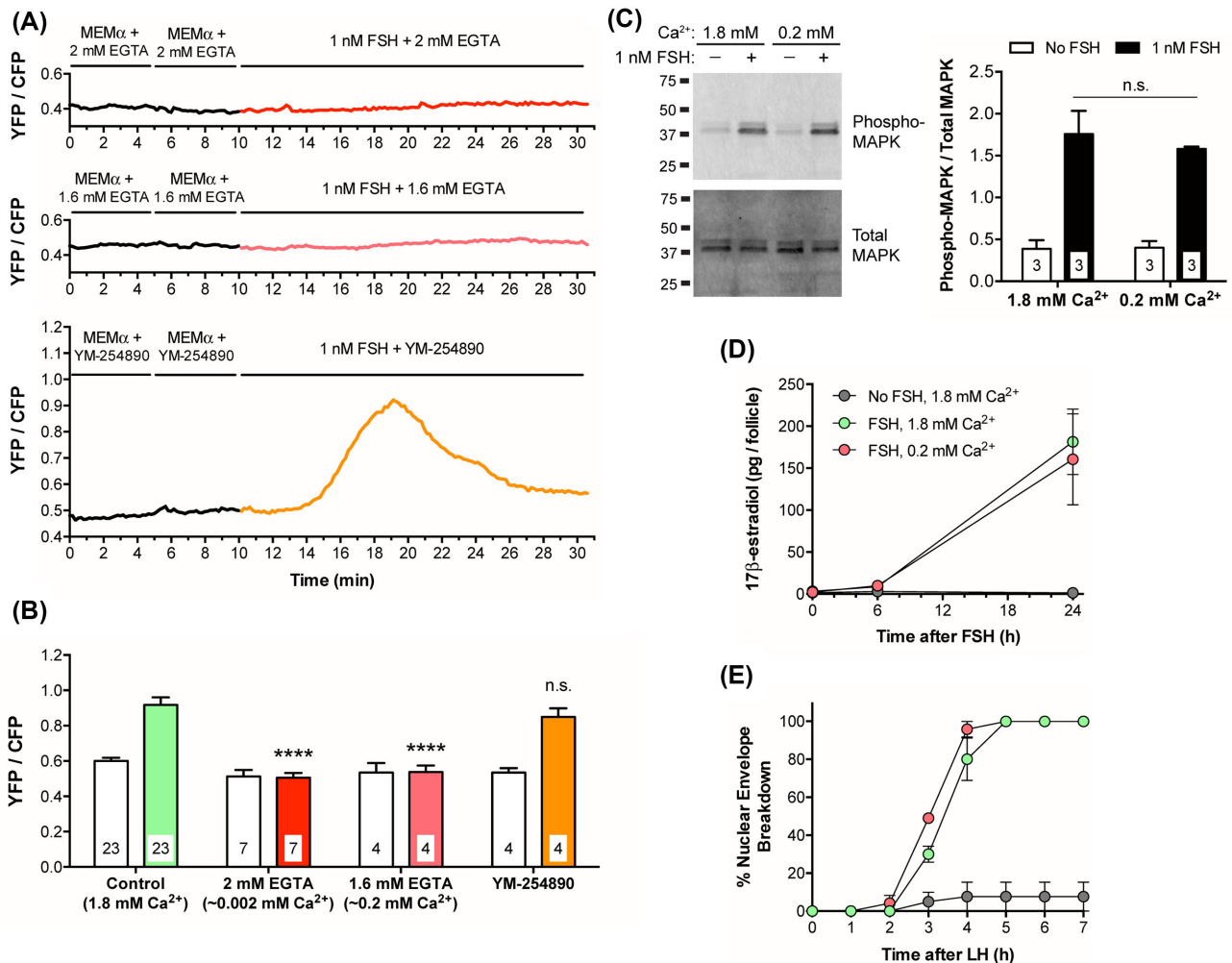
Figure 3. The FSH-induced \text{Ca}^{2+} increase in granulosa cells of intact follicles requires extracellular \text{Ca}^{2+} , but MAPK phosphorylation, 17\beta -estradiol production, and LH-induced NEBD occur independently of the \text{Ca}^{2+} increase. (A) Representative traces showing no FSH-induced \text{Ca}^{2+} increase in follicles (220–250 \mu\text{m} diameter) in media with low extracellular \text{Ca}^{2+} , and no effect of the \text{G}_q -family G-protein inhibitor YM-254 890 (10 \mu\text{M} ) on the FSH-induced \text{Ca}^{2+} increase. MEM \alpha , which contains 1.8 mM \text{CaCl}_2 , was mixed with either 2 mM EGTA (~0.002 mM free \text{Ca}^{2+} ; upper panel), or 1.6 mM EGTA (~0.2 mM free \text{Ca}^{2+} ; middle panel). Follicles were pre-incubated for ~20 min in these EGTA solutions, or for 60 min in YM-254 890 (lower panel), before addition of FSH. (B) Peak YFP/CFP ratios before and after perfusion of 1 nM FSH in the presence of varying extracellular \text{Ca}^{2+} concentrations, buffered by EGTA addition as in A, or in the presence of YM-254 890 (10 \mu\text{M} ). The ability of YM-254 890 to inhibit LH-induced \text{Ca}^{2+} elevation (see Figures 4E and 6A, B below) served as a positive control for the permeability of this inhibitor. Open bars indicate the peak YFP/CFP ratio after MEM \alpha perfusion; filled bars indicate peak YFP/CFP ratio following FSH perfusion. Following two-way ANOVA, the peak ratios following FSH perfusion in each group were compared to the control (green) bar by t -tests with the Dunnett correction for multiple comparisons; **** indicates P < 0.0001 , n.s. indicates P > 0.05 . None of the peak ratios measured during MEM \alpha perfusion (open bars) were significantly different from the control (all P > 0.05 ). (C) FSH-induced MAPK phosphorylation occurs independently of extracellular \text{Ca}^{2+} . Left: Representative western blot for phospho- and total MAPK in lysates of 180–250 \mu\text{m} follicles incubated for 20–30 min in medium with either 1.8 mM or 0.2 mM \text{Ca}^{2+} (prepared as in A), and then for 20 min in these same media with or without 1 nM FSH. Right: Ratio of phospho-/total MAPK from 3 independent experiments; n.s. indicates P > 0.05 by unpaired t -test. (D) FSH-induced estradiol production occurs independently of extracellular \text{Ca}^{2+} . 290–360 \mu\text{m} follicles were incubated with 1 nM FSH in media containing either 1.8 mM or 0.2 mM \text{Ca}^{2+} . Medium samples were collected at the indicated times for estradiol analysis. Each point represents three experiments using 14–20 follicles for each treatment. (E) FSH-induced acquisition of LH responsiveness occurs independently of extracellular \text{Ca}^{2+} . 290–360 \mu\text{m} follicles were incubated for 24 h with 1 nM FSH in media with either 1.8 mM or 0.2 mM \text{Ca}^{2+} ; 10 nM LH was then added to each dish and the time course of NEBD was determined. Each point represents three experiments using 12–19 follicles for each condition. Same legend as in (D). Values in (B–E) represent mean \pm s.e.m.
