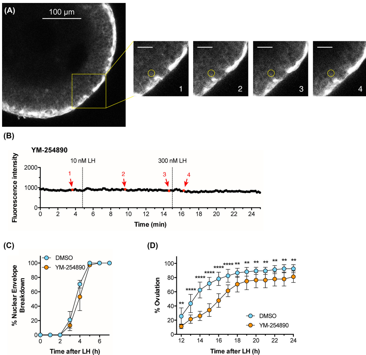
Figure 6. The G_q -family G-protein inhibitor YM-254 890 prevents \text{Ca}^{2+} oscillations in response to LH, and delays ovulation. Experiments were performed using follicles 290–360 \mu\text{m} in diameter that had been cultured for \sim 24 h in the presence of 1 nM FSH. (A, B) A follicle expressing GCaMP6s was pre-incubated with 10 \mu\text{M} YM-254 890 for 60 min before adding 10 nM LH. The yellow box outlines an area for which enlarged images are shown at four time points: before LH (image 1), after perfusion of 10 nM LH (images 2 and 3), and after perfusion of 300 nM LH (image 4); scale bar = 25 \mu\text{m} . The yellow circle (10 \mu\text{m} in diameter) indicates a mural granulosa cell for which the fluorescence intensity is graphed in B. Supplementary movie S6 shows the entire time series from which these images were selected. Representative of 3 follicles. (C, D) Inhibition of G_q -family G-proteins by preincubation of follicles with 10 \mu\text{M} YM-254 890 for 60 min before addition of 10 nM LH does not inhibit NEBD, but does delay ovulation. Graphs in C and D show the mean \pm s.e.m. of 3 and 4 experiments, respectively, with 10–18 follicles each. Data in (D) were analyzed by repeated measures two-way ANOVA, with the Holm-Sidak correction for multiple comparisons applied to the t-tests between the DMSO and YM-254 890 groups at each time point; ** indicates P < 0.01 and **** indicates P < 0.0001 .
