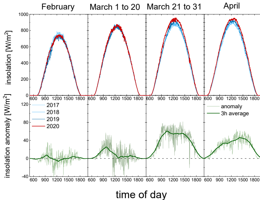
Figure 2. Reconstructed Clear-Sky Insolation and Insolation Anomaly
