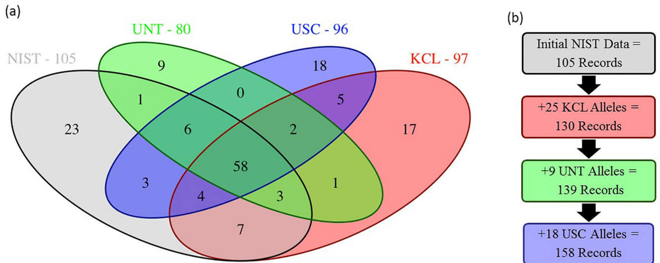
Figure 1. (a) Venn diagram demonstrating the overlap of D12S391 sequence-based alleles observed among the four laboratories, and the total number of unique sequence-based alleles observed within each laboratory. (b) Submission strategy for 158 unique sequence-based alleles observed at the D12S391 locus. The 105 unique alleles generated at NIST form the basis of STRSeq records. Subsequent submissions from KCL, UNT, and USC will add records for sequences generated at each laboratory for which records do not already exist (25, 9, and 18 records, respectively).
