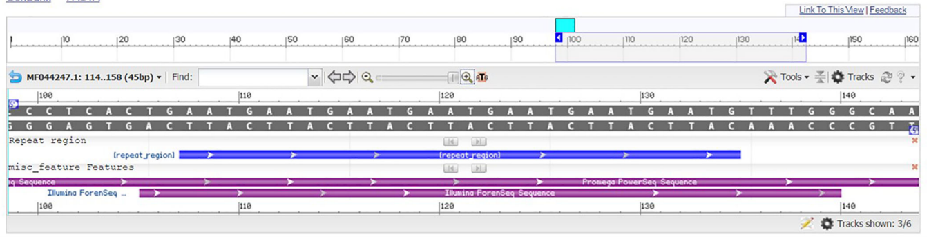
Figure 3. Example Graphics view of STRSeq Genbank record, available and interactive online at https://www.ncbi.nlm.nih.gov/nucore/1197990967?report=graph .
