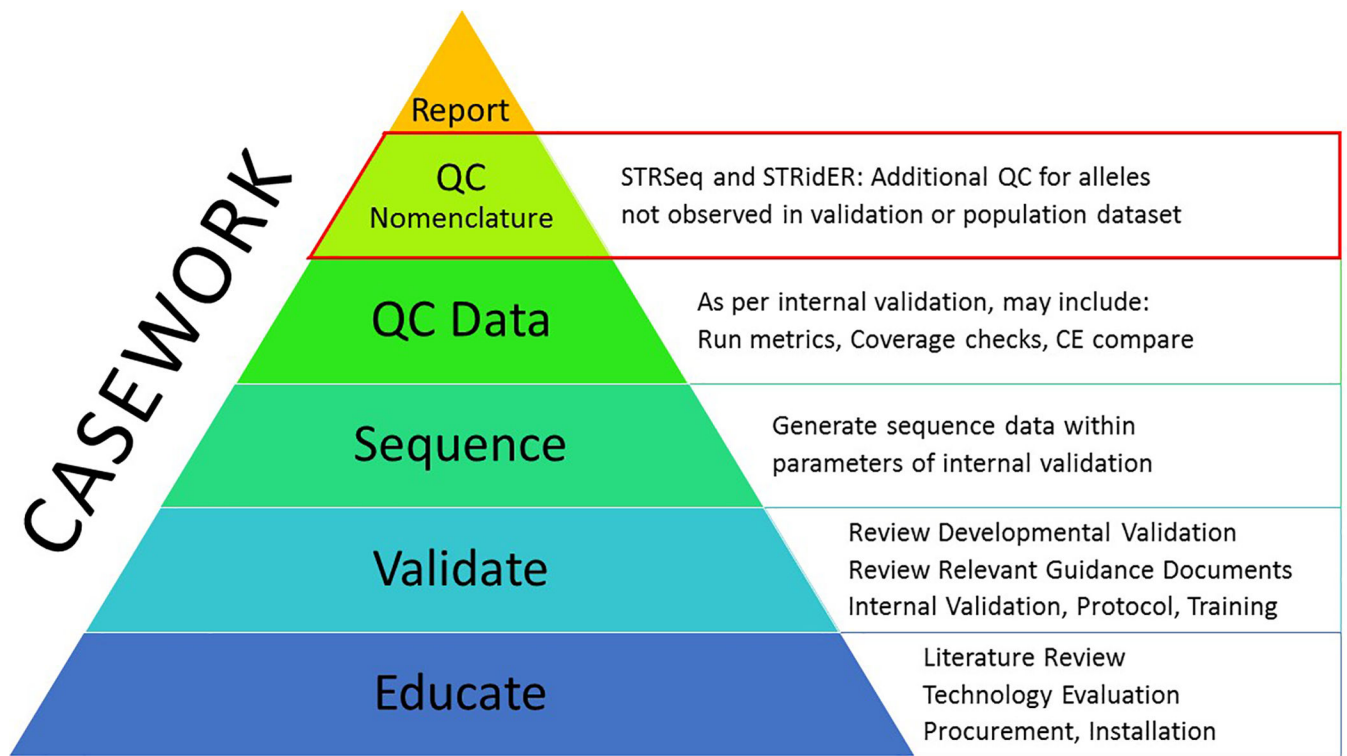
Figure 4. Outline of the anticipated STRSeq use cases for evaluation of rare alleles in forensic casework, integrated into an overall quality assurance system.
