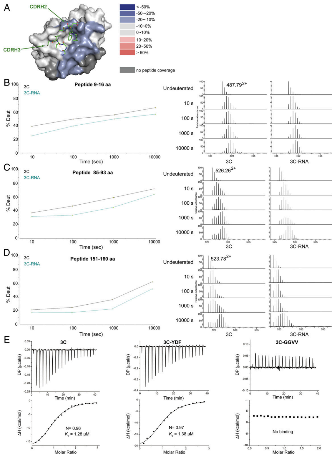
Fig. 4. GGVV blocks HRV14 3C binding to HRV genomic RNA. (A) The structure of HRV14 3C is shown as a surface representation, onto which the HDX difference heat map for HRV14 3C in complex with 72-nt RNA compared to the apo form is mapped. For heat-map color coding, red indicates increased HDX and blue indicates decreased HDX in 3C-RNA relative to apo 3C, light gray indicates no significant changes, and dark gray represents regions that were not detected in the HDX experiment. CDRH2 and CDRH3 of GGVV are shown as green stick models to illustrate the paratopes of GGVV. (B–D) Deuterium uptake plots and mass spectra of indicated peptides from HRV14 3C in the absence and presence of 72-nt RNA. Note that the HDX in peptides 9 to 16, 85 to 93, and 151 to 160 decreased considerably in the presence of 72-nt RNA, suggesting that residues in these peptides are located at the interface between HRV14 3C and 72-nt RNA. (Left) The deuterium uptake data are plotted as percent deuterium uptake versus time on a logarithmic scale. (Right) Mass spectra of indicated peptides at different labeling time points, with the mass spectra of undeuterated samples shown as controls. (E) ITC results of RNA titrated into 3C protease, 3C-YDF complex, and 3C-GGVV complex clearly demonstrate that the interaction between HRV14 3C and the 5' NCR of HRV genomic RNA is completely abrogated in the presence of GGVV.
