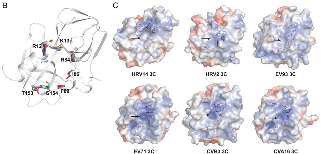
Fig. 5. Key residues on 3C involved in both GGVV and genomic RNA interactions are conserved across a panel of enteroviruses. (A) Sequence alignment of HRV14 3C with its orthologs from HRV2, EV93, EV71, CVB3, and CVA16. The secondary structure of HRV14 3C is shown above the sequence and the three critical active-site residues are indicated with orange stars. Residues on HRV14 3C involved in both GGVV and 72-nt RNA binding are marked by red triangles, and residues involved in GGVV binding but not 72-nt RNA binding are marked by light gray triangles. (B) The structure of HRV14 3C (gray) is shown as a cartoon representation onto which its orthologs from HRV2 (PDB ID code 5FX5), EV93 (PDB ID code 3Q3X), EV71 (PDB ID code 3SJK), CVB3 (PDB ID code 2ZT2), and CVA16 (PDB ID code 3SJB) are superimposed. The backbone of the residues that are marked by red triangle in A are shown as stick models to highlight their structural conservation in space across HRV14 (gray), HRV2 (cyan), EV93 (orange), EV71 (green), CVB3 (blue), and CVA16 (hot pink). (C) The 3C proteases from HRV14, HRV2, EV93, EV71, CVB3, and CVA16 were rendered as an electrostatic surface representation (−5 to +5 kT/e), where hydrophobic surfaces are in whitish gray, basic in blue, and acidic in red. The residues marked by red triangle in A are shown as stick-and-ball models. Note that these residues are located around a similar pocket (marked with an arrow) on 3C in all six structures.
