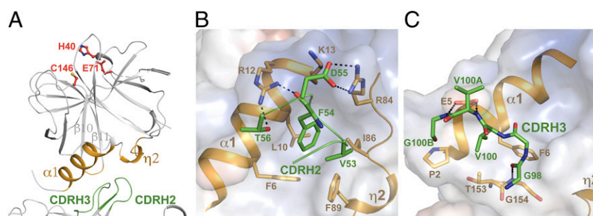
Fig. 3. GGVV binds HRV14 3C only with two heavy-chain CDRs. (A) The protein–protein interfaces between HRV14 3C protease and GGVV. The three critical residues are shown as red stick models to illustrate the position of active site. HRV14 3C is shown as gray ribbons, while helix \alpha_1 , 3_{10} helix \eta_2 , and the \beta -turn between the \beta_{10} and \beta_{11} strands at the antibody–protein interface are highlighted in orange. CDRH3 and CDRH2 of GGVV that are involved in binding HRV14 3C are highlighted in green. (B and C) Close-up views of the interfaces between CDRH2 (GGVV) and HRV14 3C (B) and between CDRH3 (GGVV) and HRV14 3C (C). HRV14 3C is shown as an electrostatic surface, with helix \alpha_1 , 3_{10} helix \eta_2 , and the \beta -turn between the \beta_{10} and \beta_{11} strands as orange ribbons. Key residues that are involved in interactions at the antibody–protein interface are shown as stick models, labeled and color-coded as in A. Polar and electrostatic interactions are indicated with black dashed lines. The CDR residues of GGVV are labeled following Kabat numbering.
