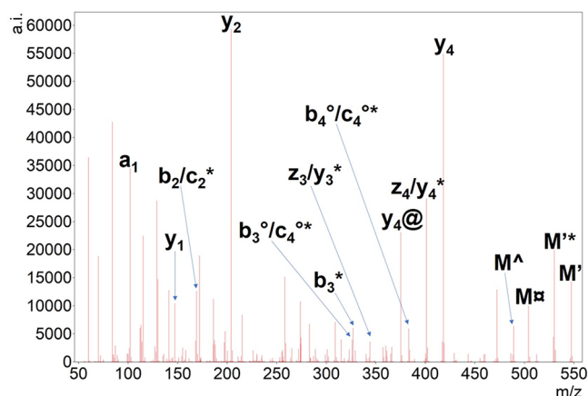
Figure 6. EThcD tandem mass spectrum of doubly protonated Ac-SGXGK histone peptide. The undetected charge-reduced precursor is only signed as M. Hydrogen atom loss is depicted as '. Neutral losses of ammonia (*), water (deg), the citrulline-selective carbamoyl radical (currency sign) or isocyanic acid (@) are also shown. Note that the spectrum is very similar to an HCD one; radical losses could be explained by even-electron fragmentation from M' as well.
