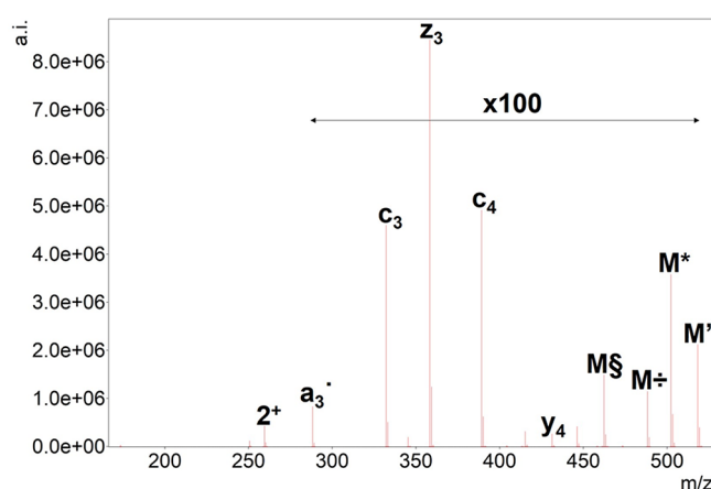
Figure 4. ETD tandem mass spectrum of doubly protonated SGR(Me)GK. Precursor ion is denoted as “2+”, and the undetected charge-reduced precursor is only signed as M. Hydrogen atom loss is depicted as *. Neutral losses of ammonia (*) and the \text{N}^G -methylarginine-selective methylamine (±) and N -methylcarbodiimide losses (§) are also shown. For ease of interpretation, precursor intensity is reduced to 1/100 of its original value.
