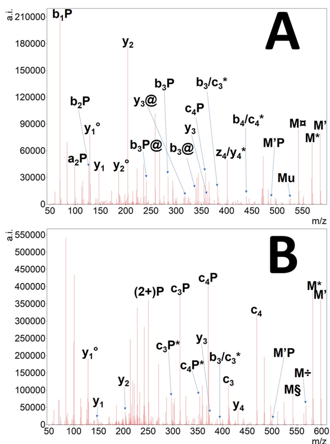
Figure 7. EThcD tandem mass spectrum of doubly protonated pSGXGK (A) and pSGR(Me)GK (B) histone peptides. The undetected charge-reduced precursor is only signed as M. Hydrogen atom loss is depicted as '. Neutral losses of ammonia (*), water (deg), the citrulline-selective carbamoyl radical (currency sign), or isocyanic acid (@) as well as the N^G -methylarginine-selective methylamine (÷) and N-methylcarbodiimide losses (§) are also shown. Note that all b_i related fragments may represent c_i^* ones, and all z_i related fragments may represent y_i^* as well.
